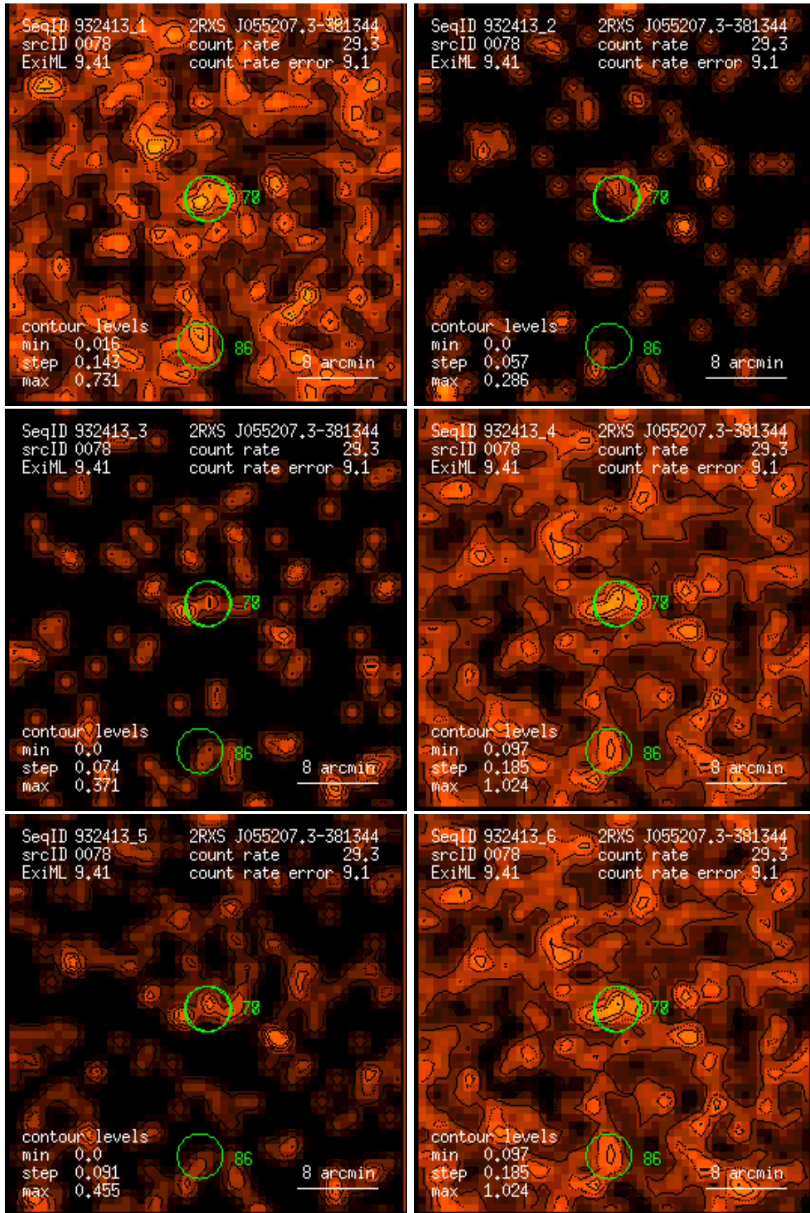
Figure 78: RASS 932413: detection 0078: band rate images, Gaussian filter: (1) PSPC channels 11 – 41, (2) 52 – 90, (3) 91 – 201, (4) 11 – 235, (5) 52 – 201, (6) 11 – 201. Broad band rates in counts/ks. Band rate contour levels in counts/ks/arcmin 2 .
