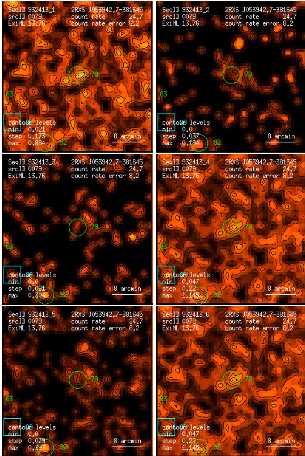
Figure 79: RASS 932413: detection 0079: band rate images, Gaussian filter: (1) PSPC channels 11 – 41, (2) 52 – 90, (3) 91 – 201, (4) 11 – 235, (5) 52 – 201, (6) 11 – 201. Broad band rates in counts/ks. Band rate contour levels in counts/ks/arcmin 2 .
