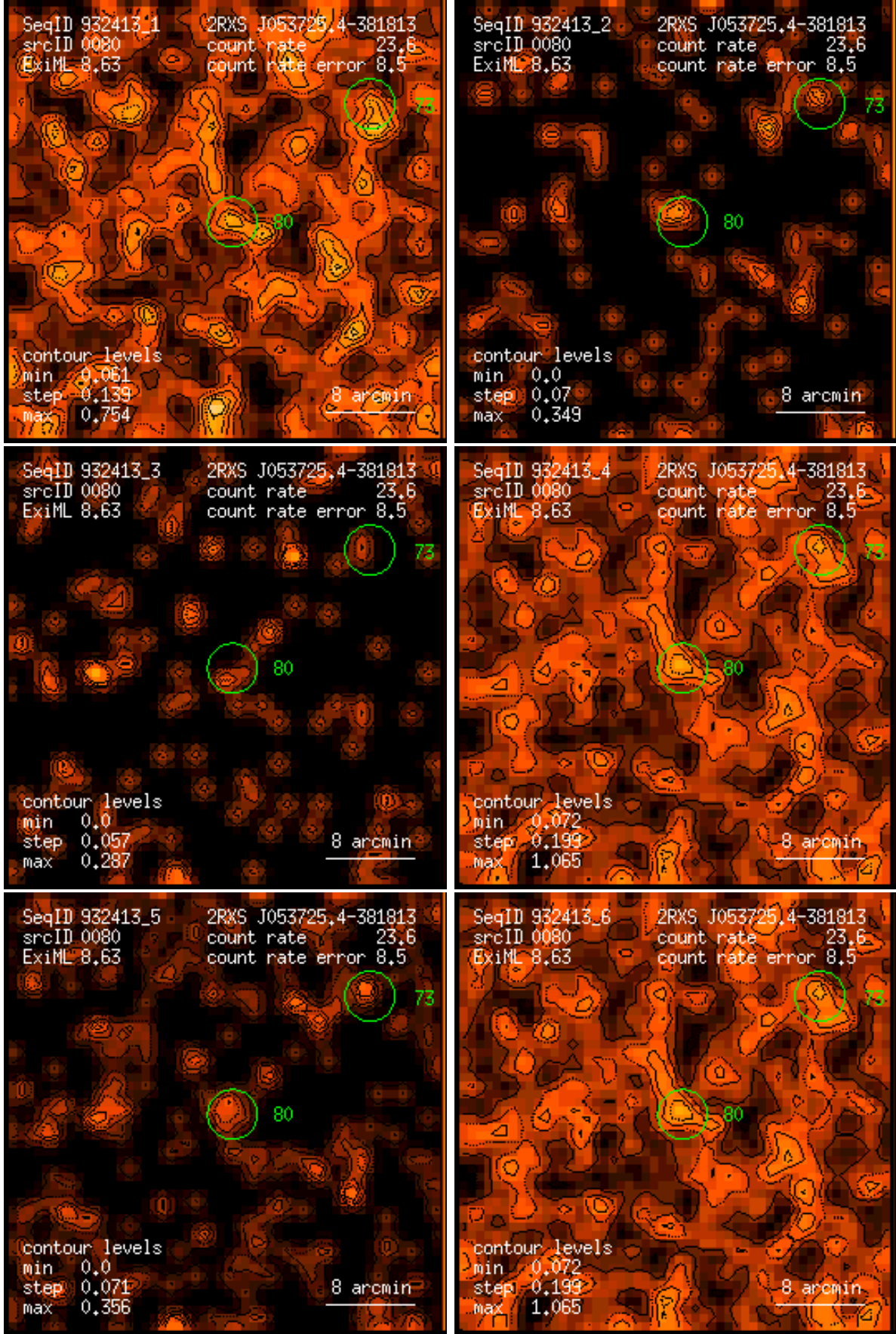
Figure 80: RASS 932413: detection 0080: band rate images, Gaussian filter: (1) PSPC channels 11 – 41, (2) 52 – 90, (3) 91 – 201, (4) 11 – 235, (5) 52 – 201, (6) 11 – 201. Broad band rates in counts/ks. Band rate contour levels in counts/ks/arcmin 2 .
