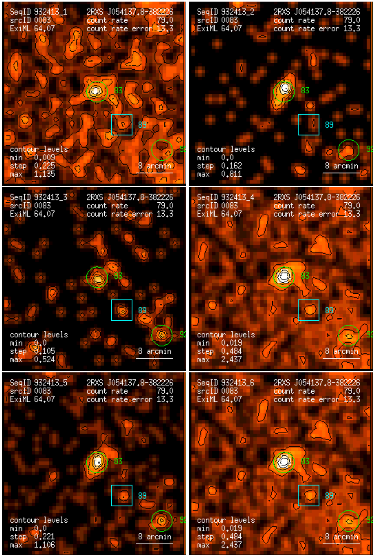
Figure 83: RASS 932413: detection 0083: band rate images, Gaussian filter: (1) PSPC channels 11 – 41, (2) 52 – 90, (3) 91 – 201, (4) 11 – 235, (5) 52 – 201, (6) 11 – 201. Broad band rates in counts/ks. Band rate contour levels in counts/ks/arcmin 2 .
