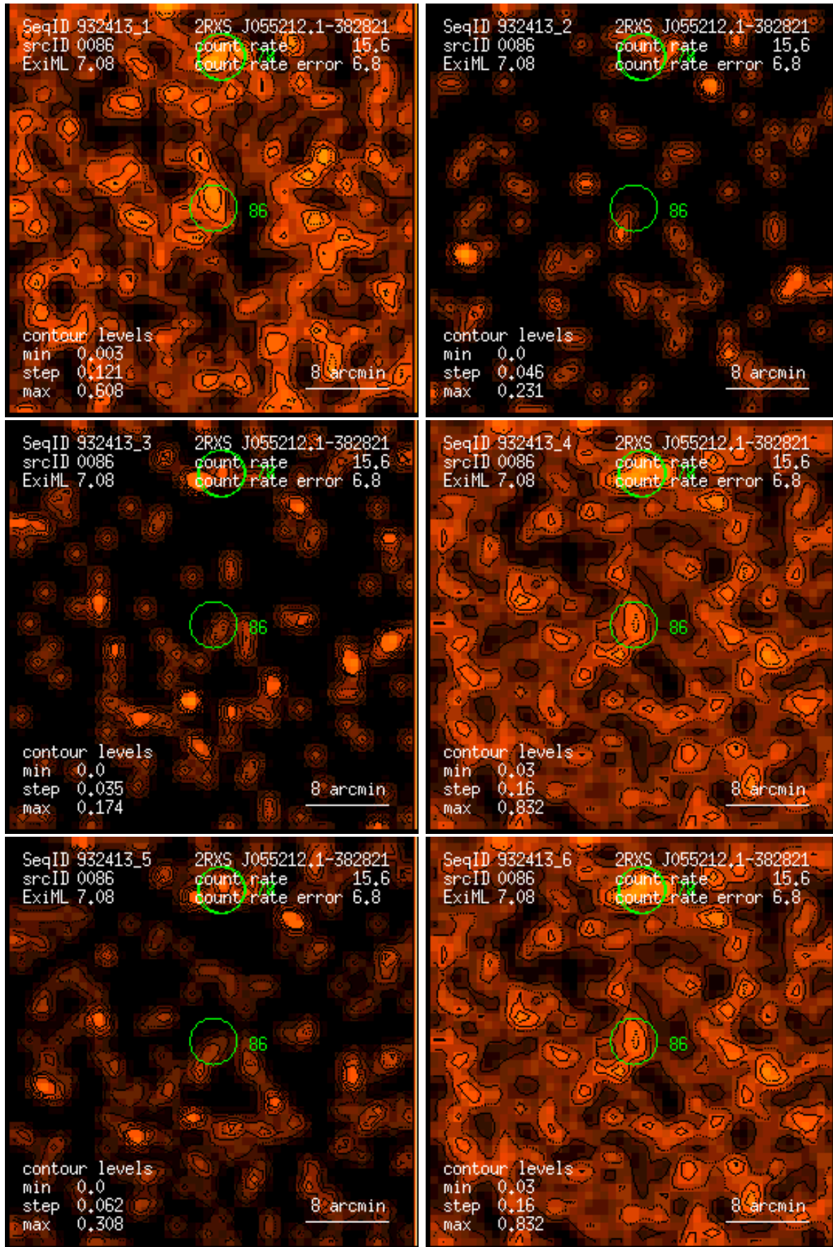
Figure 86: RASS 932413: detection 0086: band rate images, Gaussian filter: (1) PSPC channels 11 – 41, (2) 52 – 90, (3) 91 – 201, (4) 11 – 235, (5) 52 – 201, (6) 11 – 201. Broad band rates in counts/ks. Band rate contour levels in counts/ks/arcmin 2 .
