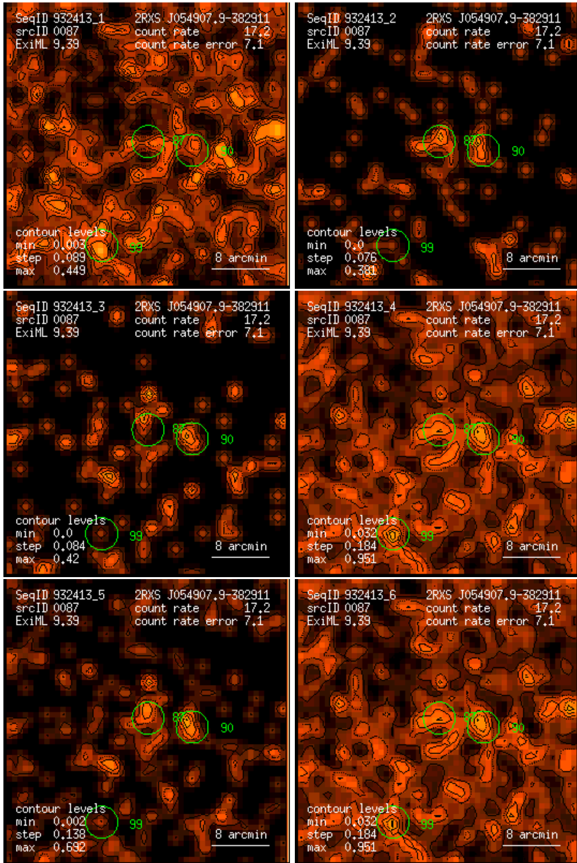
Figure 87: RASS 932413: detection 0087: band rate images, Gaussian filter: (1) PSPC channels 11 – 41, (2) 52 – 90, (3) 91 – 201, (4) 11 – 235, (5) 52 – 201, (6) 11 – 201. Broad band rates in counts/ks. Band rate contour levels in counts/ks/arcmin 2 .
