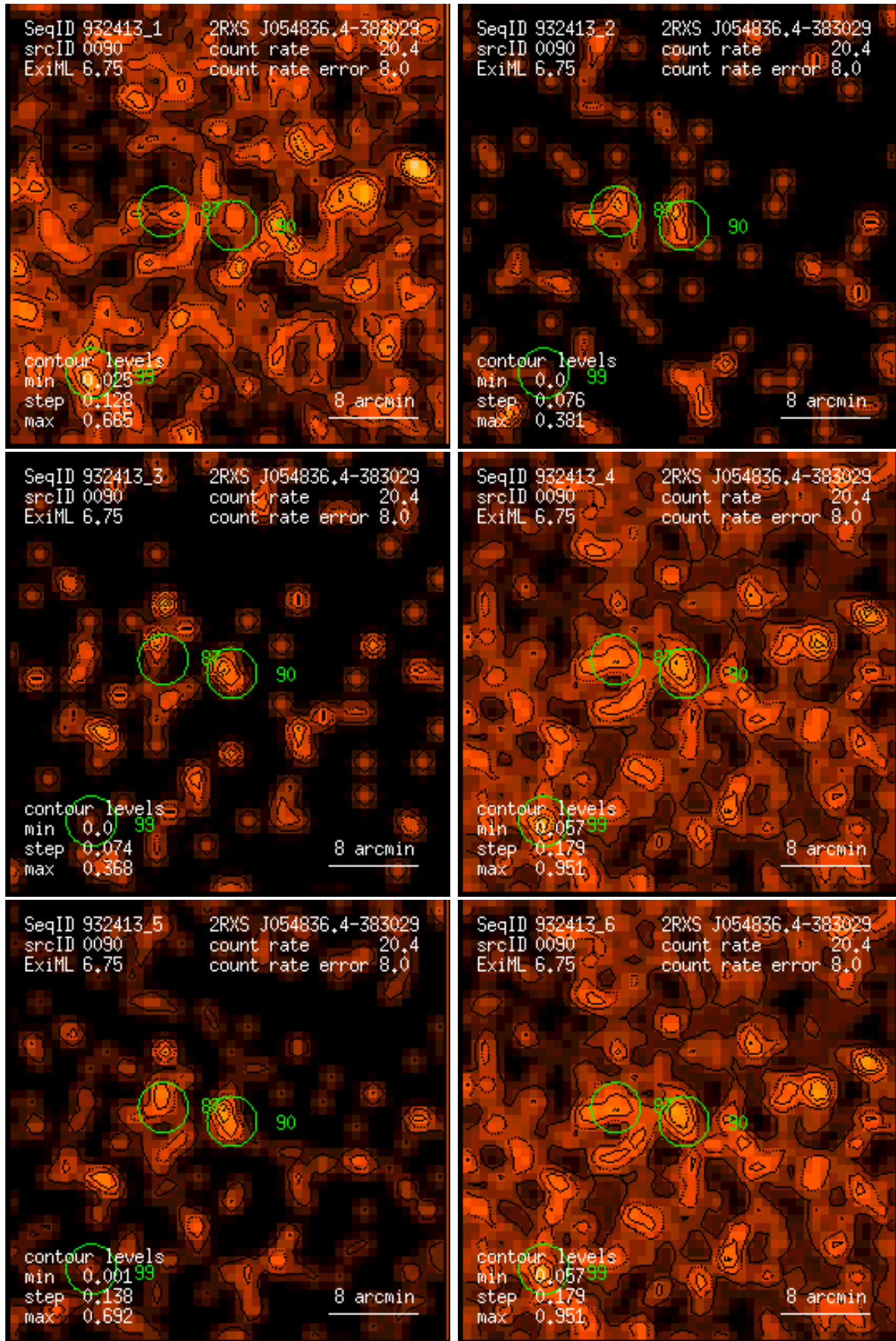
Figure 90: RASS 932413: detection 0090: band rate images, Gaussian filter: (1) PSPC channels 11 – 41, (2) 52 – 90, (3) 91 – 201, (4) 11 – 235, (5) 52 – 201, (6) 11 – 201. Broad band rates in counts/ks. Band rate contour levels in counts/ks/arcmin 2 .
