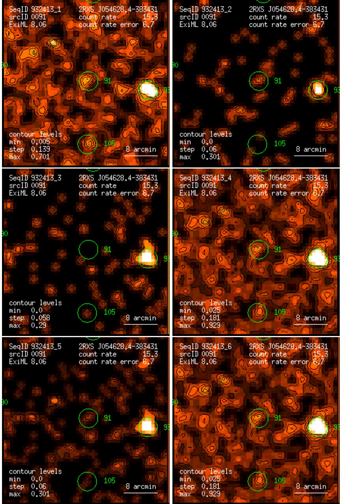
Figure 91: RASS 932413: detection 0091: band rate images, Gaussian filter: (1) PSPC channels 11 – 41, (2) 52 – 90, (3) 91 – 201, (4) 11 – 235, (5) 52 – 201, (6) 11 – 201. Broad band rates in counts/ks. Band rate contour levels in counts/ks/arcmin 2 .
