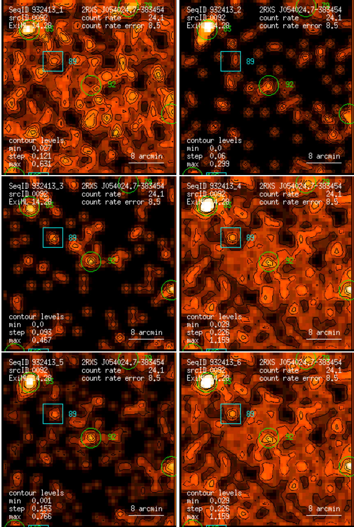
Figure 92: RASS 932413: detection 0092: band rate images, Gaussian filter: (1) PSPC channels 11 – 41, (2) 52 – 90, (3) 91 – 201, (4) 11 – 235, (5) 52 – 201, (6) 11 – 201. Broad band rates in counts/ks. Band rate contour levels in counts/ks/arcmin 2 .
