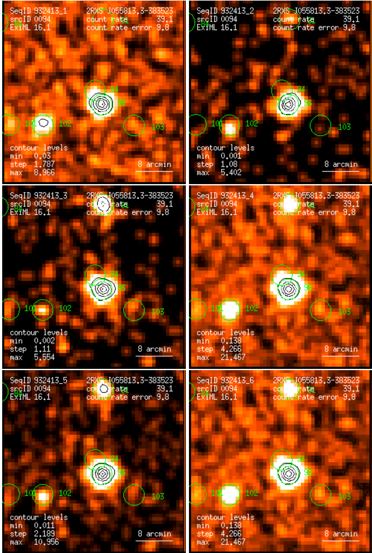
Figure 94: RASS 932413: detection 0094: band rate images, Gaussian filter: (1) PSPC channels 11 – 41, (2) 52 – 90, (3) 91 – 201, (4) 11 – 235, (5) 52 – 201, (6) 11 – 201. Broad band rates in counts/ks. Band rate contour levels in counts/ks/arcmin 2 .
