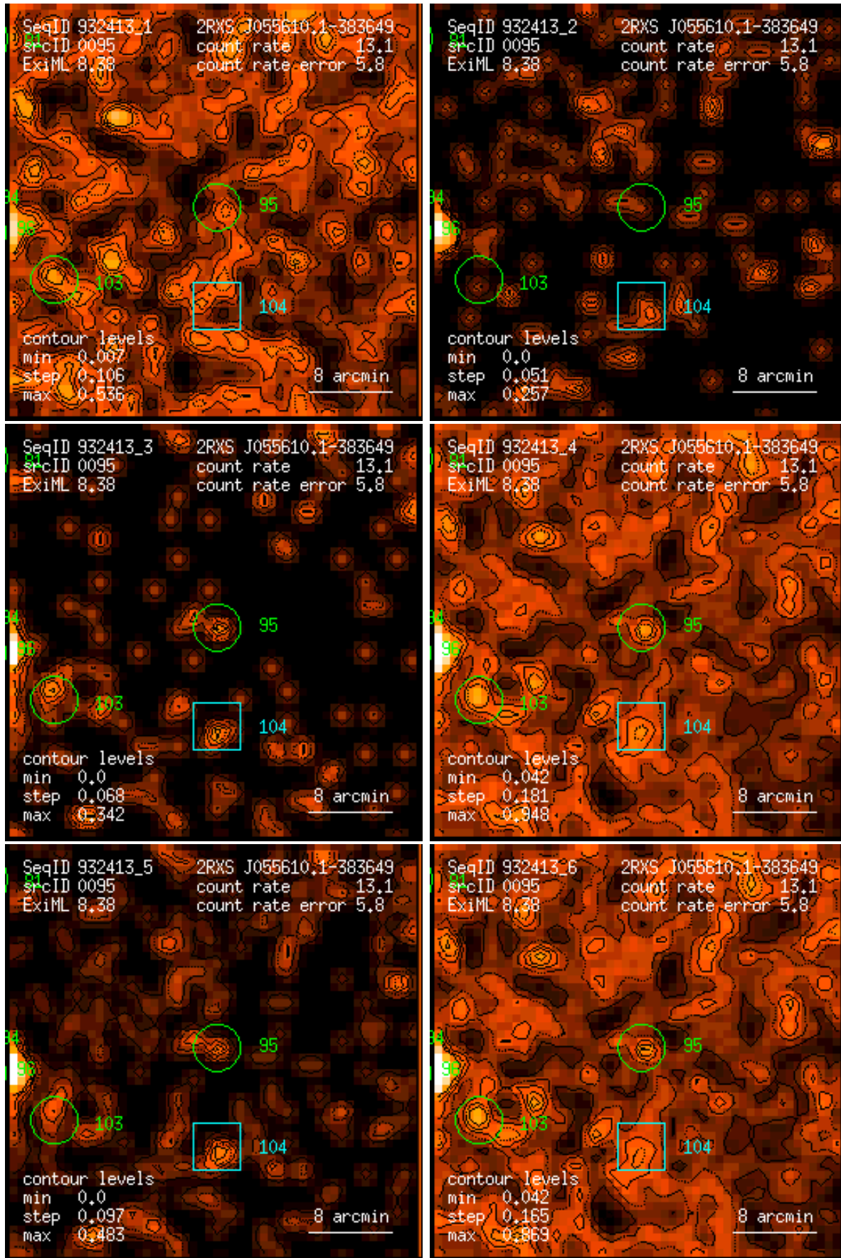
Figure 95: RASS 932413: detection 0095: band rate images, Gaussian filter: (1) PSPC channels 11 – 41, (2) 52 – 90, (3) 91 – 201, (4) 11 – 235, (5) 52 – 201, (6) 11 – 201. Broad band rates in counts/ks. Band rate contour levels in counts/ks/arcmin 2 .
