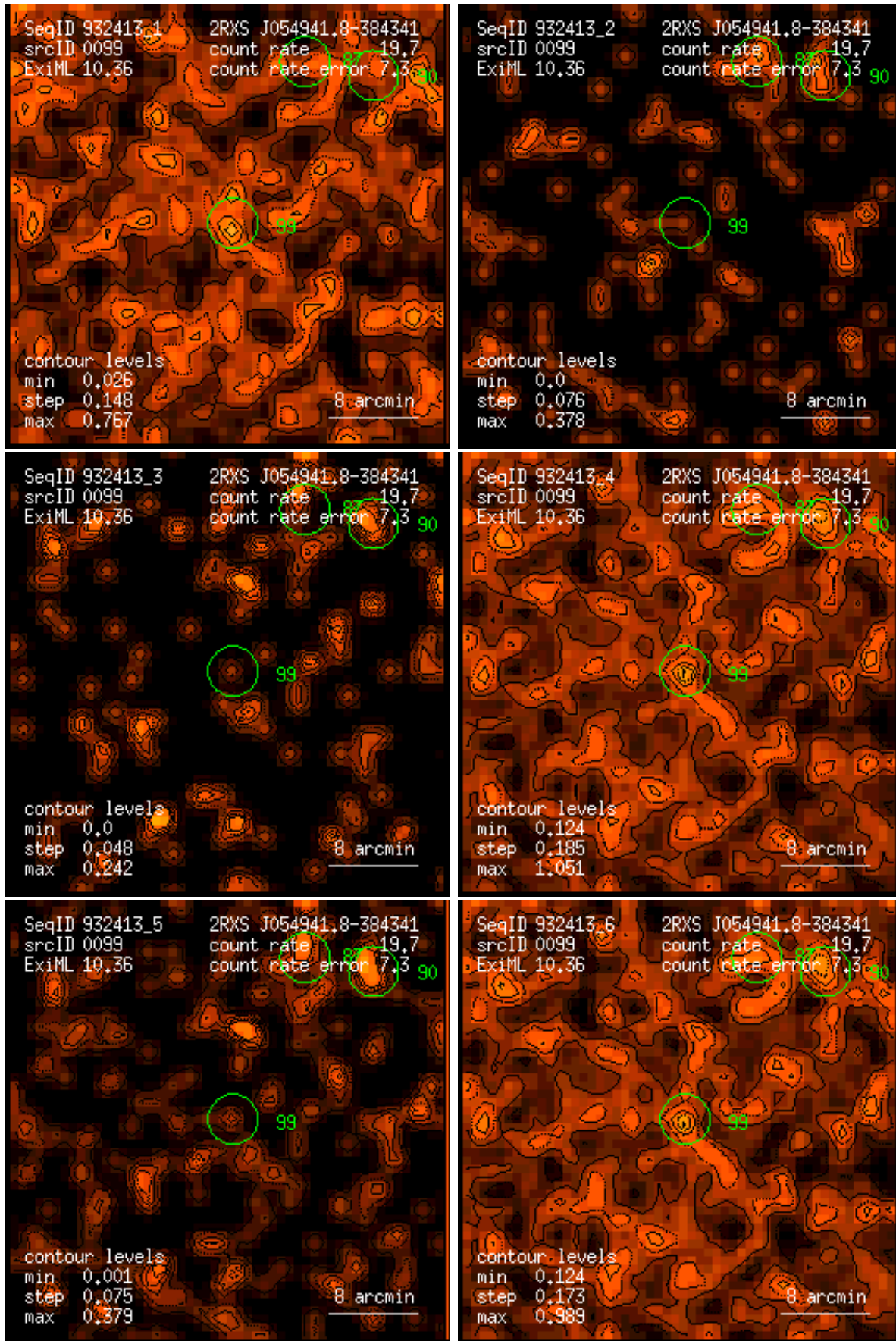
Figure 99: RASS 932413: detection 0099: band rate images, Gaussian filter: (1) PSPC channels 11 – 41, (2) 52 – 90, (3) 91 – 201, (4) 11 – 235, (5) 52 – 201, (6) 11 – 201. Broad band rates in counts/ks. Band rate contour levels in counts/ks/arcmin 2 .
