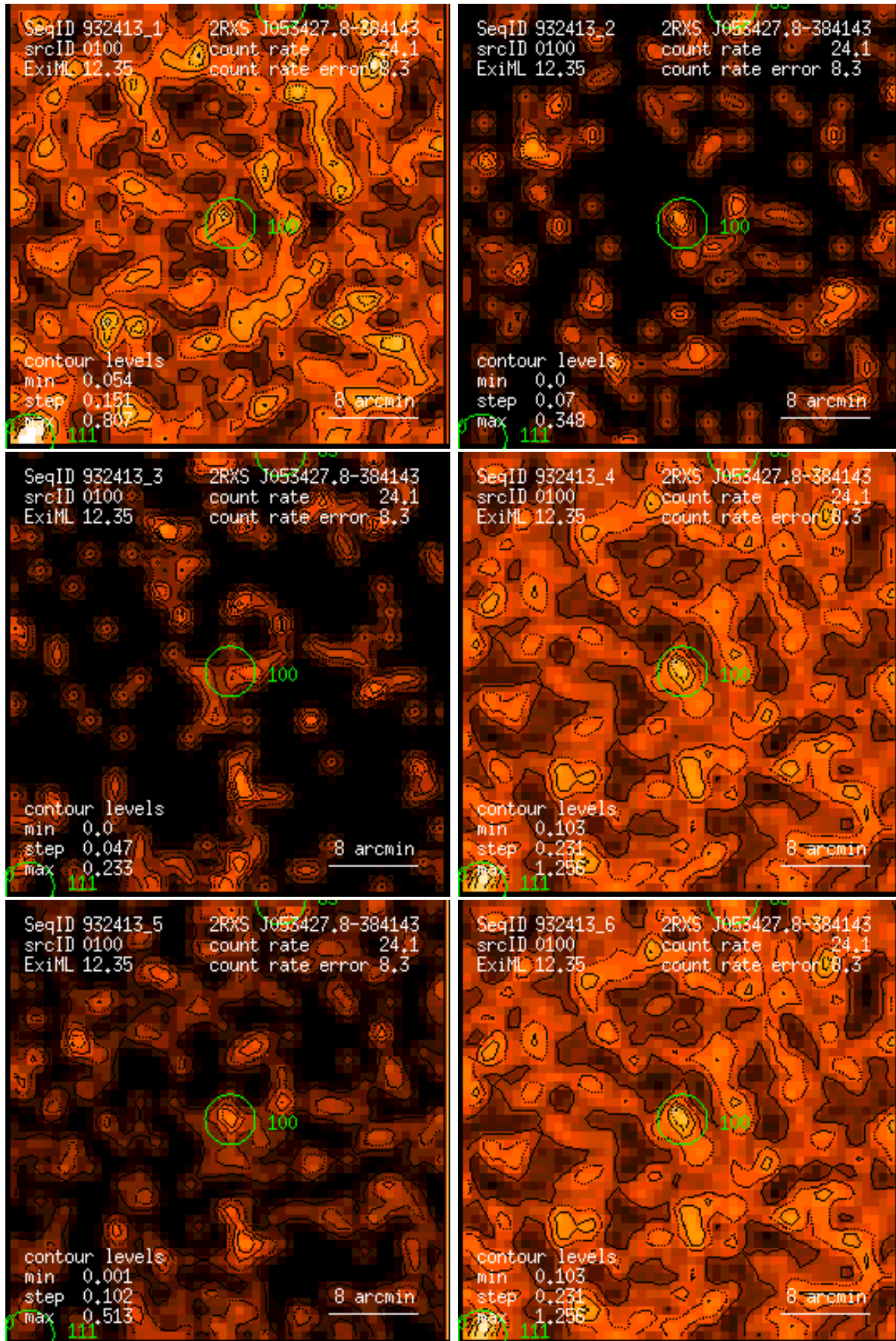
Figure 100: RASS 932413: detection 0100: band rate images, Gaussian filter: (1) PSPC channels 11 – 41, (2) 52 – 90, (3) 91 – 201, (4) 11 – 235, (5) 52 – 201, (6) 11 – 201. Broad band rates in counts/ks. Band rate contour levels in counts/ks/arcmin 2 .
