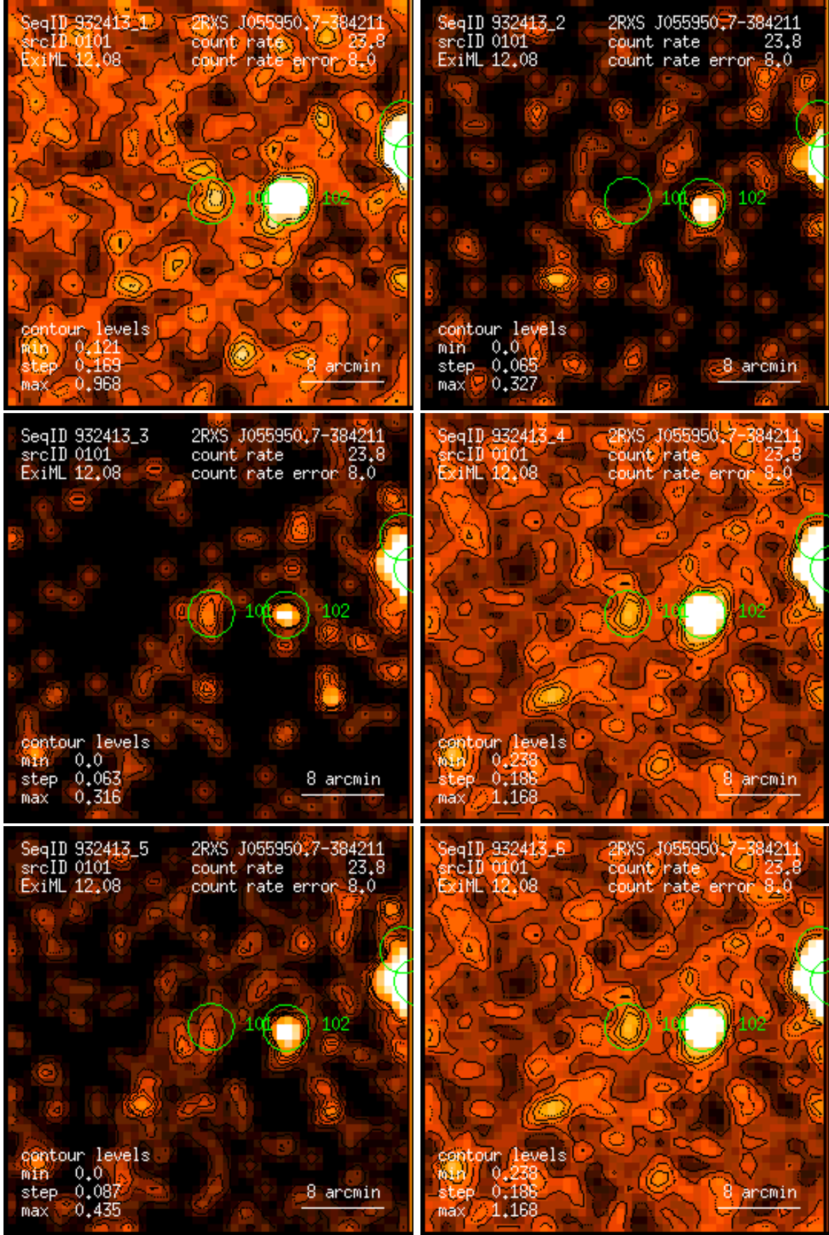
Figure 101: RASS 932413: detection 0101: band rate images, Gaussian filter: (1) PSPC channels 11 – 41, (2) 52 – 90, (3) 91 – 201, (4) 11 – 235, (5) 52 – 201, (6) 11 – 201. Broad band rates in counts/ks. Band rate contour levels in counts/ks/arcmin 2 .
