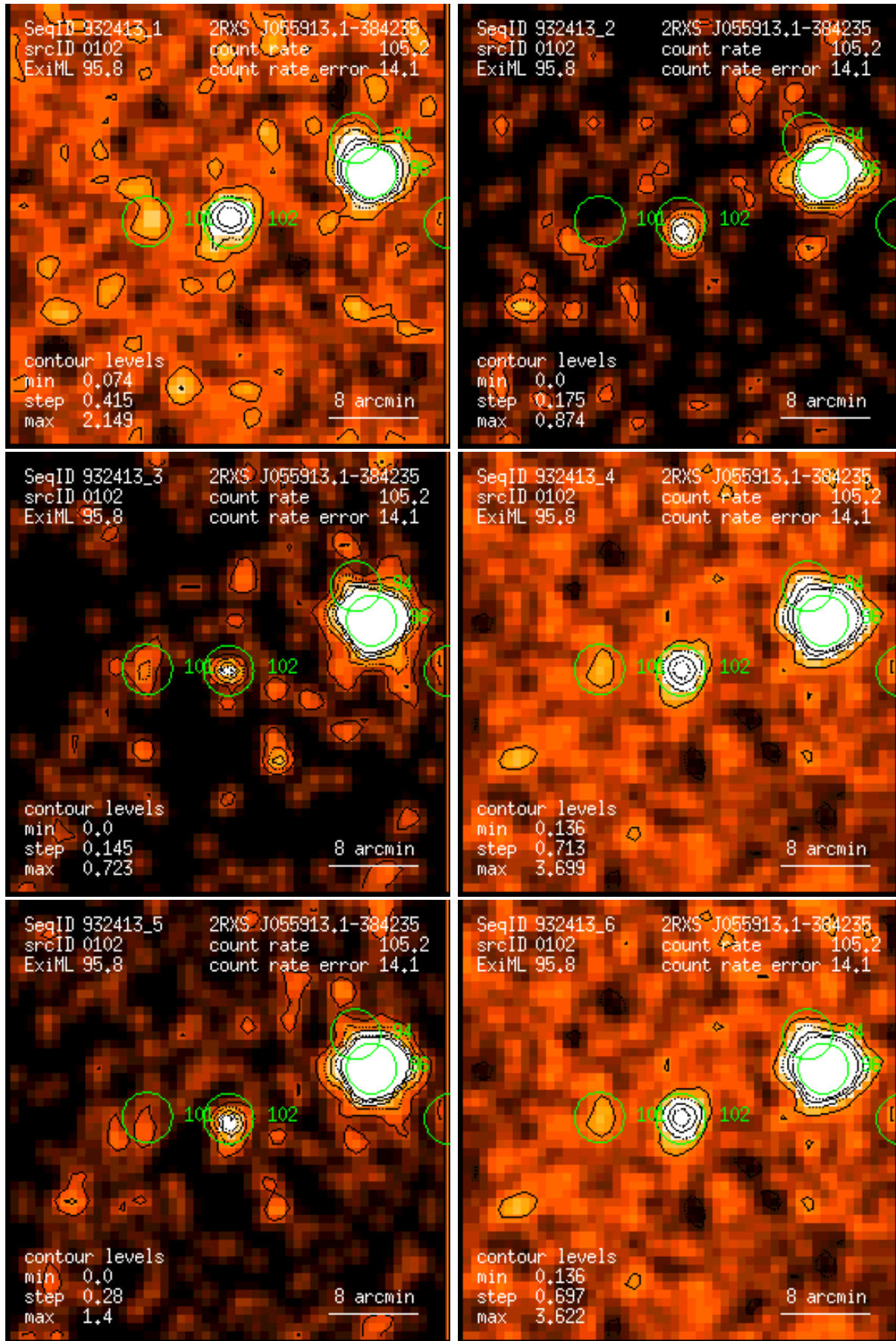
Figure 102: RASS 932413: detection 0102: band rate images, Gaussian filter: (1) PSPC channels 11 – 41, (2) 52 – 90, (3) 91 – 201, (4) 11 – 235, (5) 52 – 201, (6) 11 – 201. Broad band rates in counts/ks. Band rate contour levels in counts/ks/arcmin 2 .
