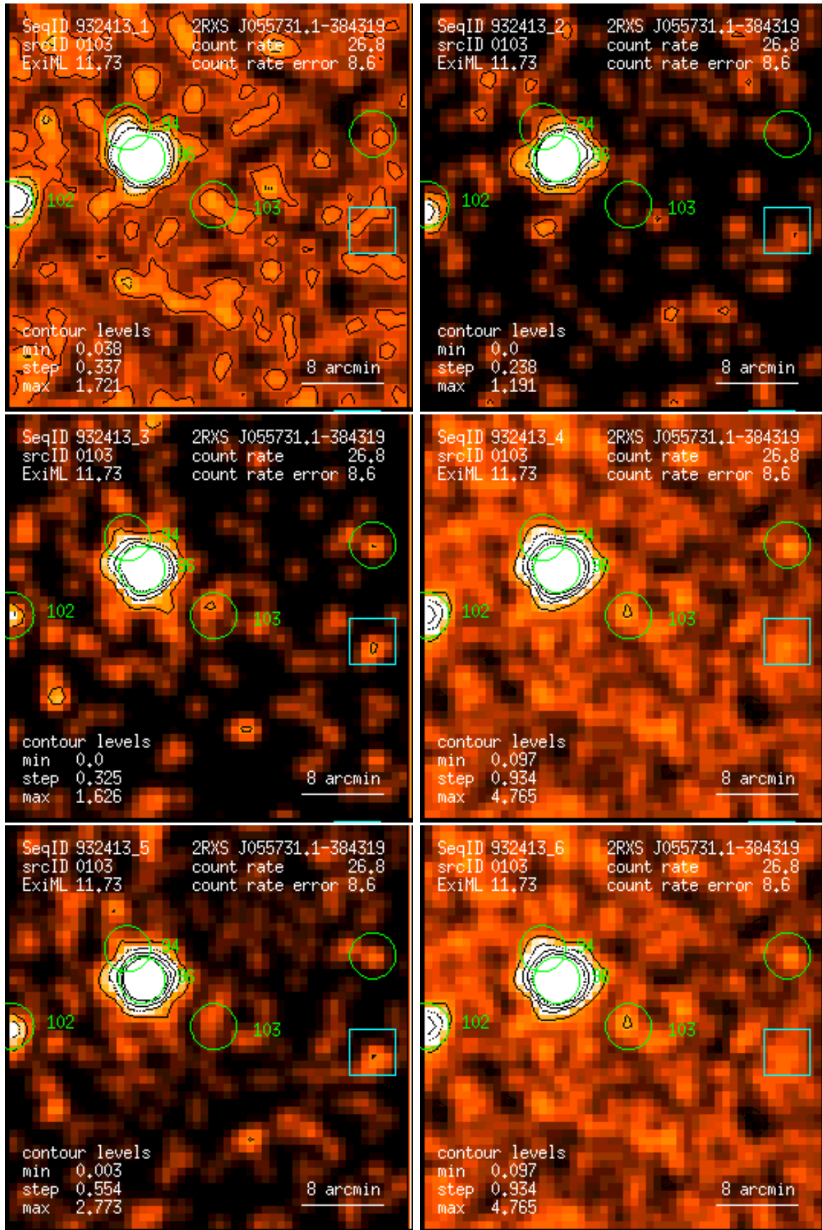
Figure 103: RASS 932413: detection 0103: band rate images, Gaussian filter: (1) PSPC channels 11 – 41, (2) 52 – 90, (3) 91 – 201, (4) 11 – 235, (5) 52 – 201, (6) 11 – 201. Broad band rates in counts/ks. Band rate contour levels in counts/ks/arcmin 2 .
