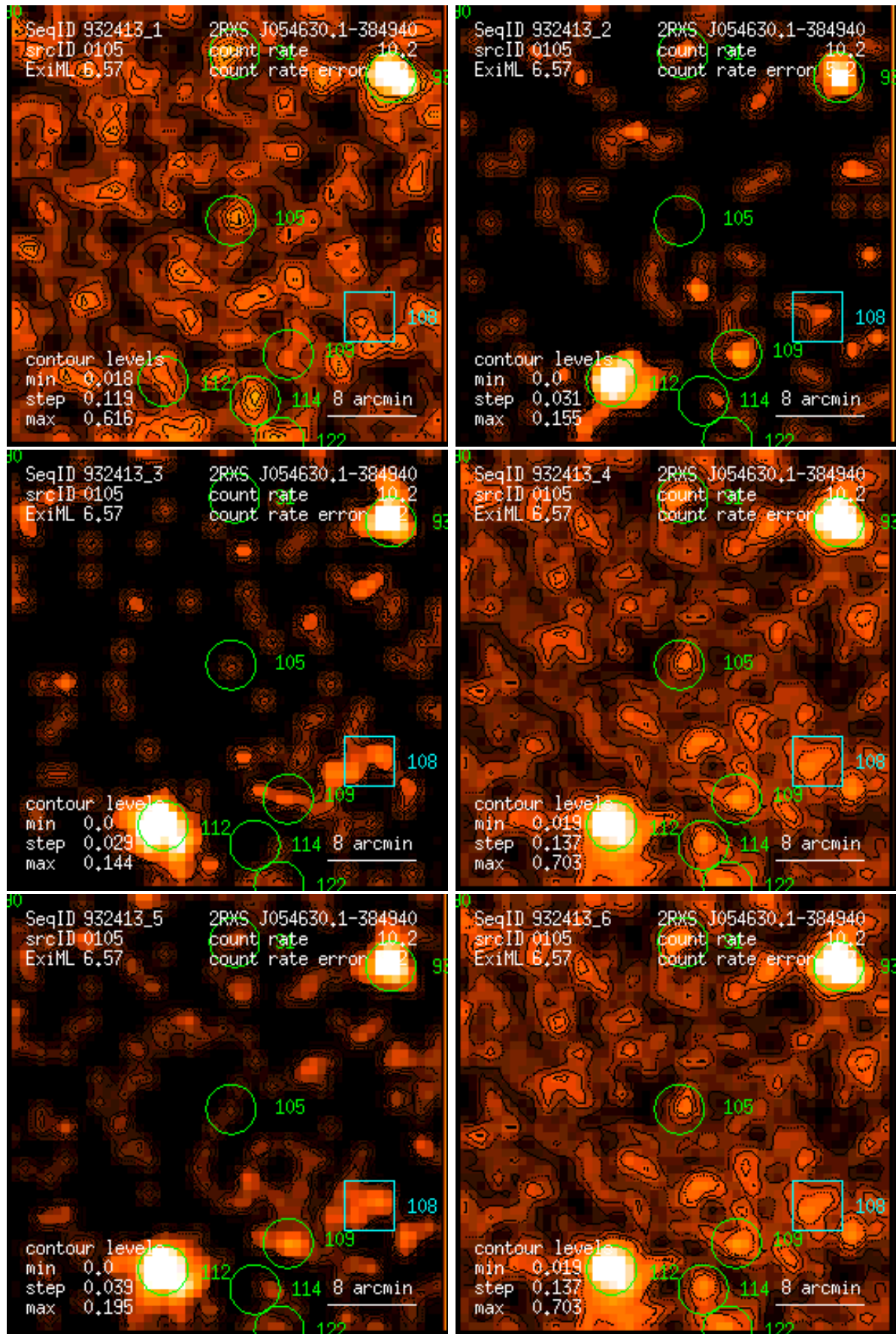
Figure 105: RASS 932413: detection 0105: band rate images, Gaussian filter: (1) PSPC channels 11 – 41, (2) 52 – 90, (3) 91 – 201, (4) 11 – 235, (5) 52 – 201, (6) 11 – 201. Broad band rates in counts/ks. Band rate contour levels in counts/ks/arcmin 2 .
