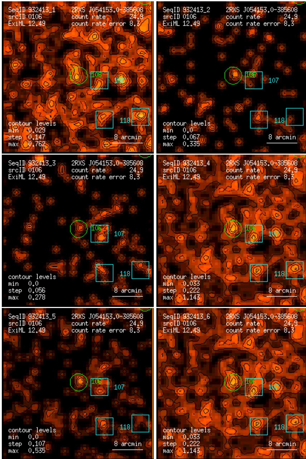
Figure 106: RASS 932413: detection 0106: band rate images, Gaussian filter: (1) PSPC channels 11 – 41, (2) 52 – 90, (3) 91 – 201, (4) 11 – 235, (5) 52 – 201, (6) 11 – 201. Broad band rates in counts/ks. Band rate contour levels in counts/ks/arcmin 2 .
