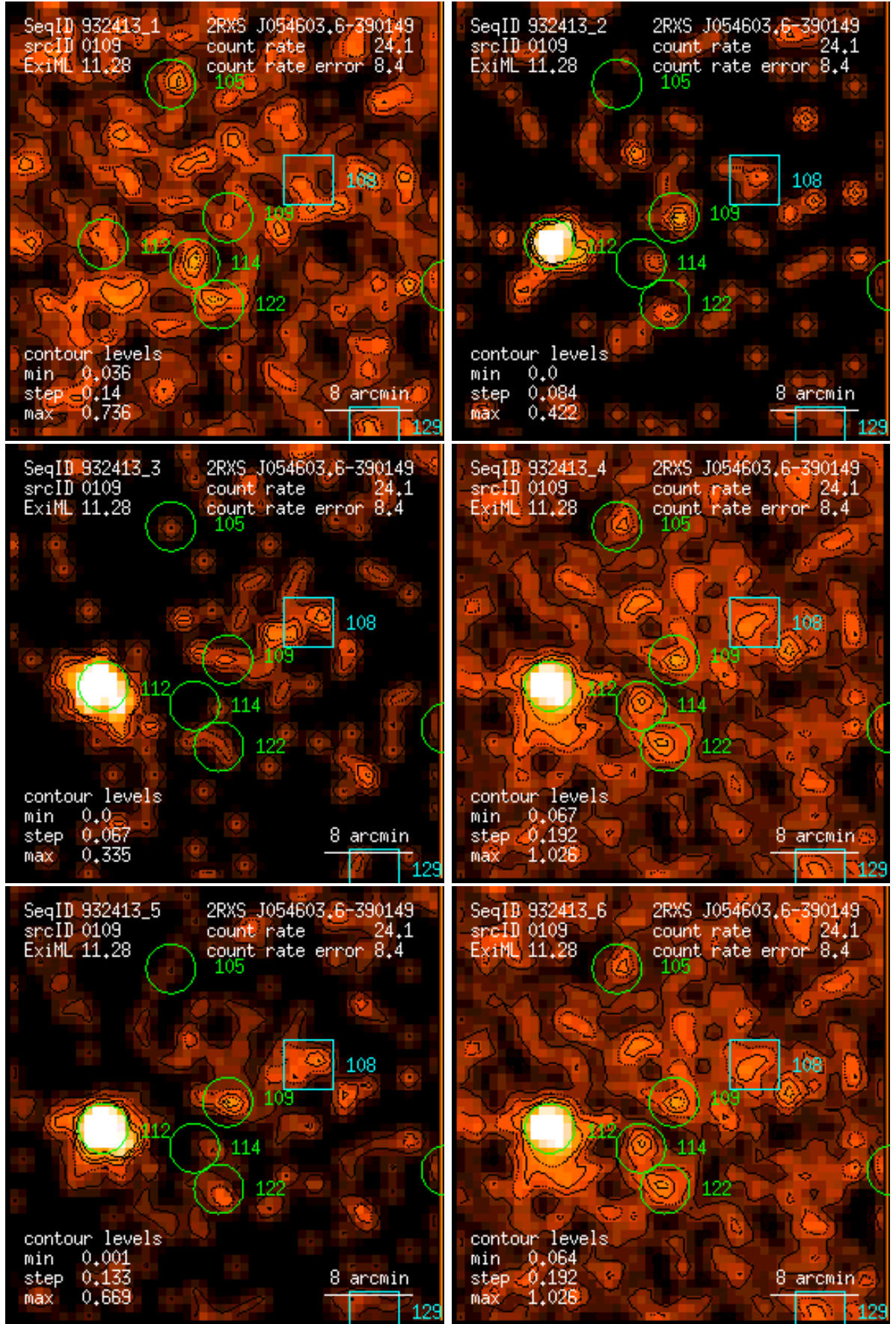
Figure 109: RASS 932413: detection 0109: band rate images, Gaussian filter: (1) PSPC channels 11 – 41, (2) 52 – 90, (3) 91 – 201, (4) 11 – 235, (5) 52 – 201, (6) 11 – 201. Broad band rates in counts/ks. Band rate contour levels in counts/ks/arcmin 2 .
