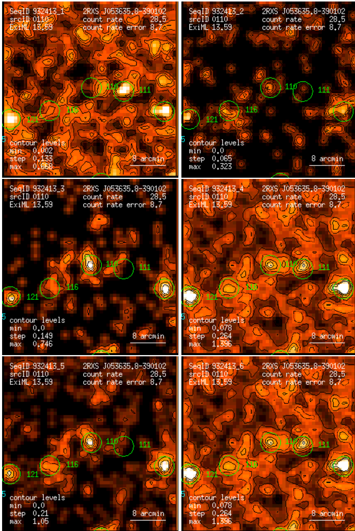
Figure 110: RASS 932413: detection 0110: band rate images, Gaussian filter: (1) PSPC channels 11 – 41, (2) 52 – 90, (3) 91 – 201, (4) 11 – 235, (5) 52 – 201, (6) 11 – 201. Broad band rates in counts/ks. Band rate contour levels in counts/ks/arcmin 2 .
