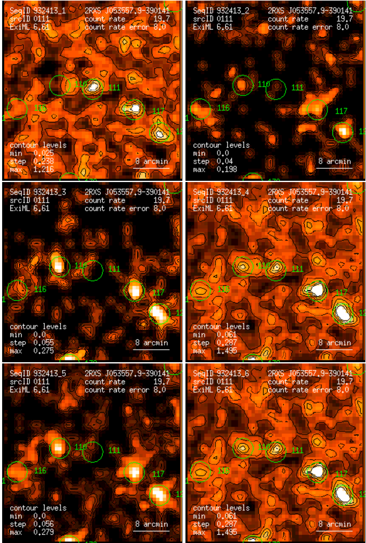
Figure 111: RASS 932413: detection 0111: band rate images, Gaussian filter: (1) PSPC channels 11 – 41, (2) 52 – 90, (3) 91 – 201, (4) 11 – 235, (5) 52 – 201, (6) 11 – 201. Broad band rates in counts/ks. Band rate contour levels in counts/ks/arcmin 2 .
