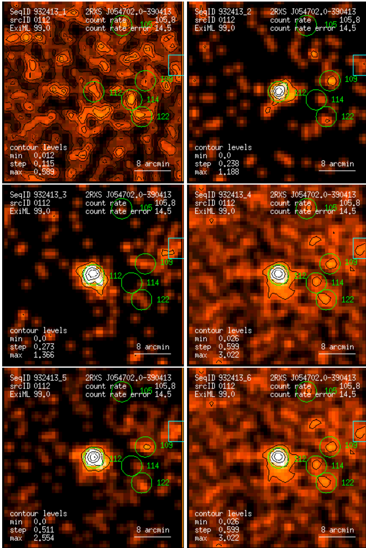
Figure 112: RASS 932413: detection 0112: band rate images, Gaussian filter: (1) PSPC channels 11 – 41, (2) 52 – 90, (3) 91 – 201, (4) 11 – 235, (5) 52 – 201, (6) 11 – 201. Broad band rates in counts/ks. Band rate contour levels in counts/ks/arcmin 2 .
