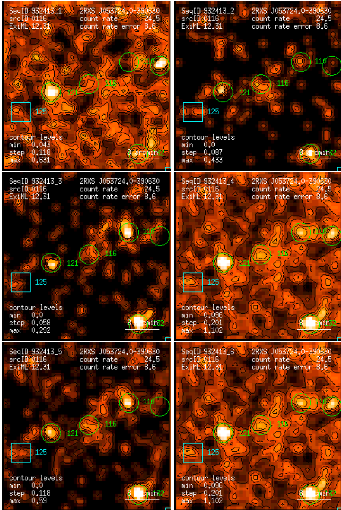
Figure 116: RASS 932413: detection 0116: band rate images, Gaussian filter: (1) PSPC channels 11 – 41, (2) 52 – 90, (3) 91 – 201, (4) 11 – 235, (5) 52 – 201, (6) 11 – 201. Broad band rates in counts/ks. Band rate contour levels in counts/ks/arcmin 2 .
