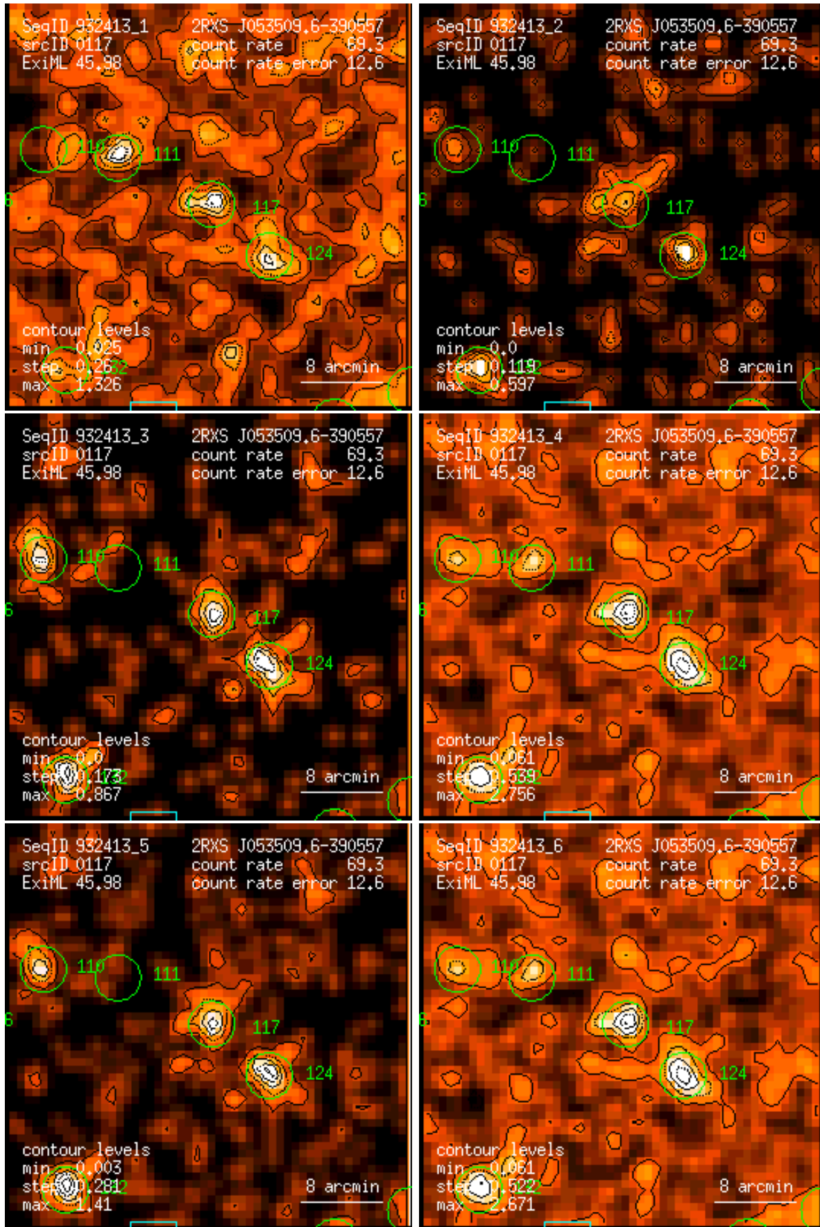
Figure 117: RASS 932413: detection 0117: band rate images, Gaussian filter: (1) PSPC channels 11 – 41, (2) 52 – 90, (3) 91 – 201, (4) 11 – 235, (5) 52 – 201, (6) 11 – 201. Broad band rates in counts/ks. Band rate contour levels in counts/ks/arcmin 2 .
