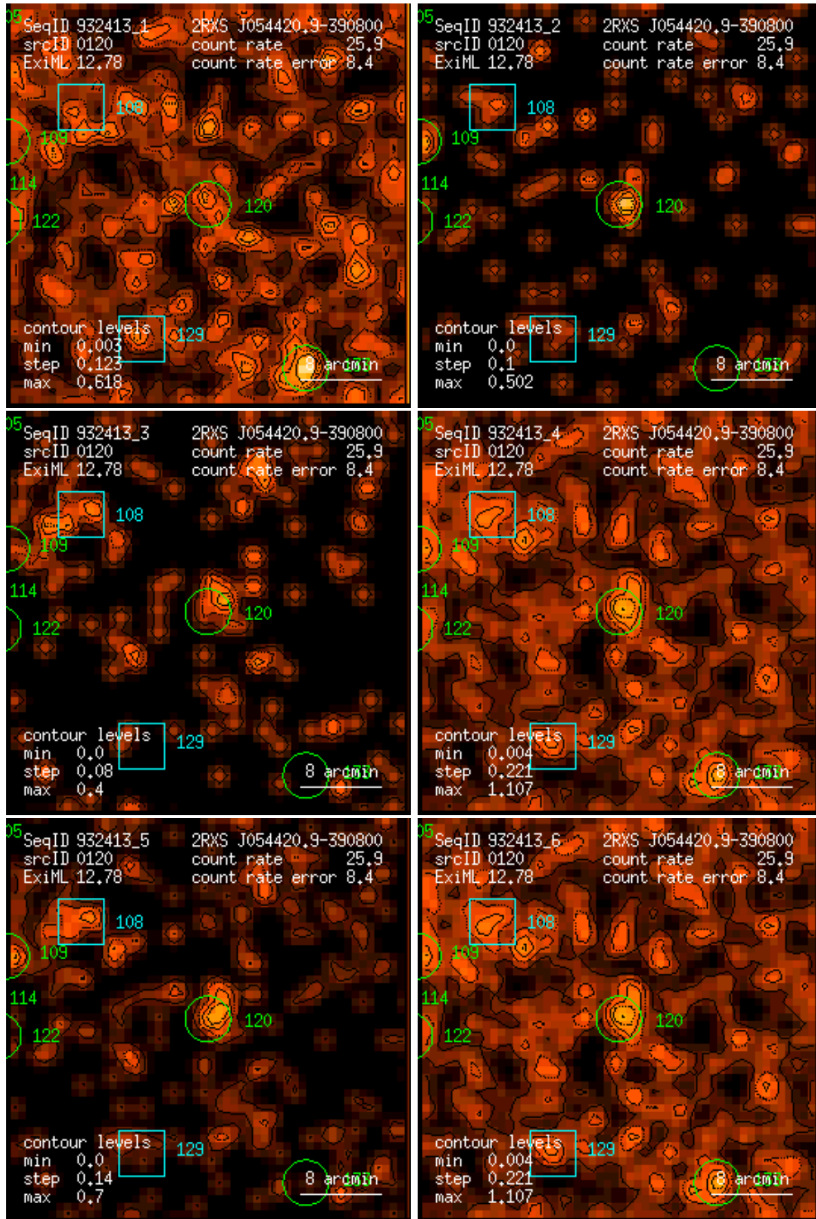
Figure 120: RASS 932413: detection 0120: band rate images, Gaussian filter: (1) PSPC channels 11 – 41, (2) 52 – 90, (3) 91 – 201, (4) 11 – 235, (5) 52 – 201, (6) 11 – 201. Broad band rates in counts/ks. Band rate contour levels in counts/ks/arcmin 2 .
