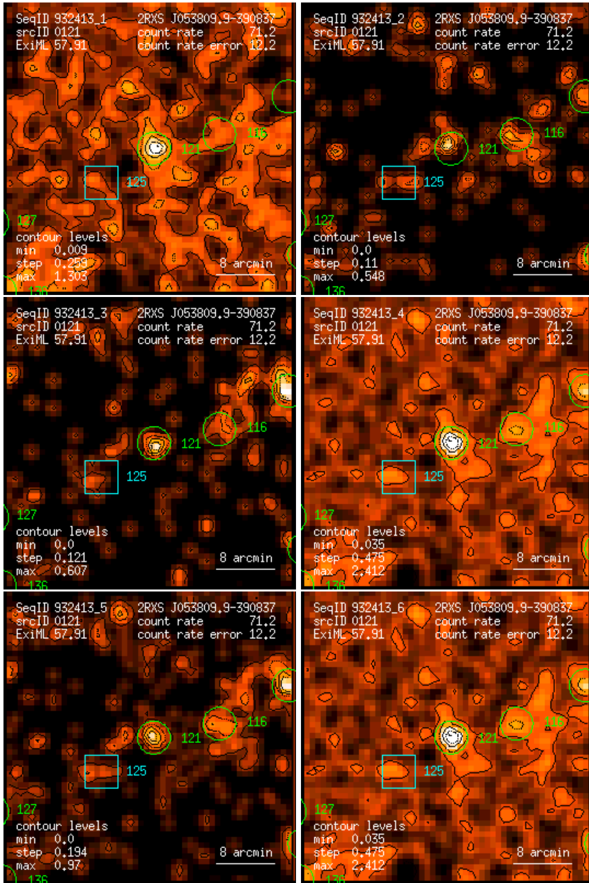
Figure 121: RASS 932413: detection 0121: band rate images, Gaussian filter: (1) PSPC channels 11 – 41, (2) 52 – 90, (3) 91 – 201, (4) 11 – 235, (5) 52 – 201, (6) 11 – 201. Broad band rates in counts/ks. Band rate contour levels in counts/ks/arcmin 2 .
