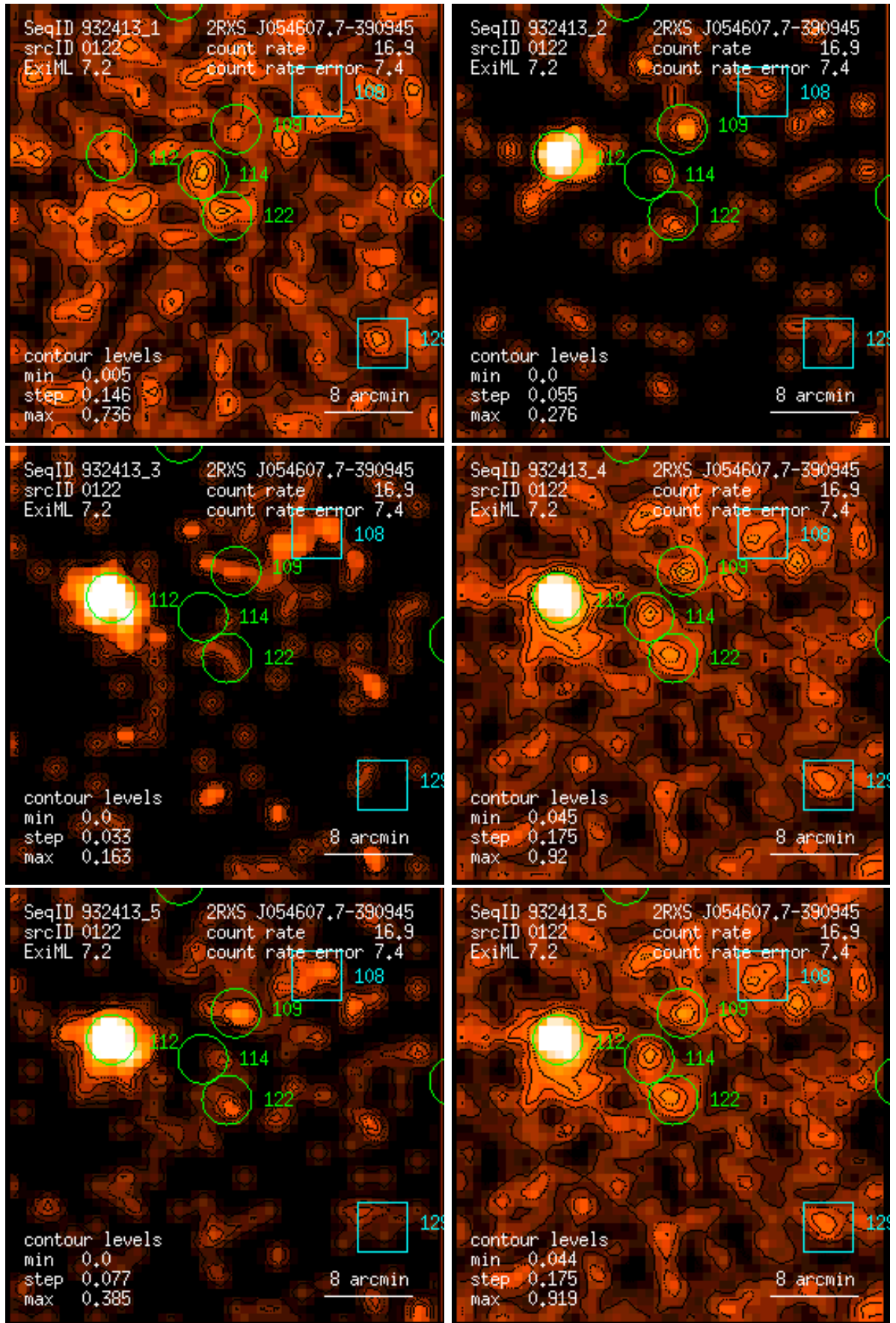
Figure 122: RASS 932413: detection 0122: band rate images, Gaussian filter: (1) PSPC channels 11 – 41, (2) 52 – 90, (3) 91 – 201, (4) 11 – 235, (5) 52 – 201, (6) 11 – 201. Broad band rates in counts/ks. Band rate contour levels in counts/ks/arcmin 2 .
