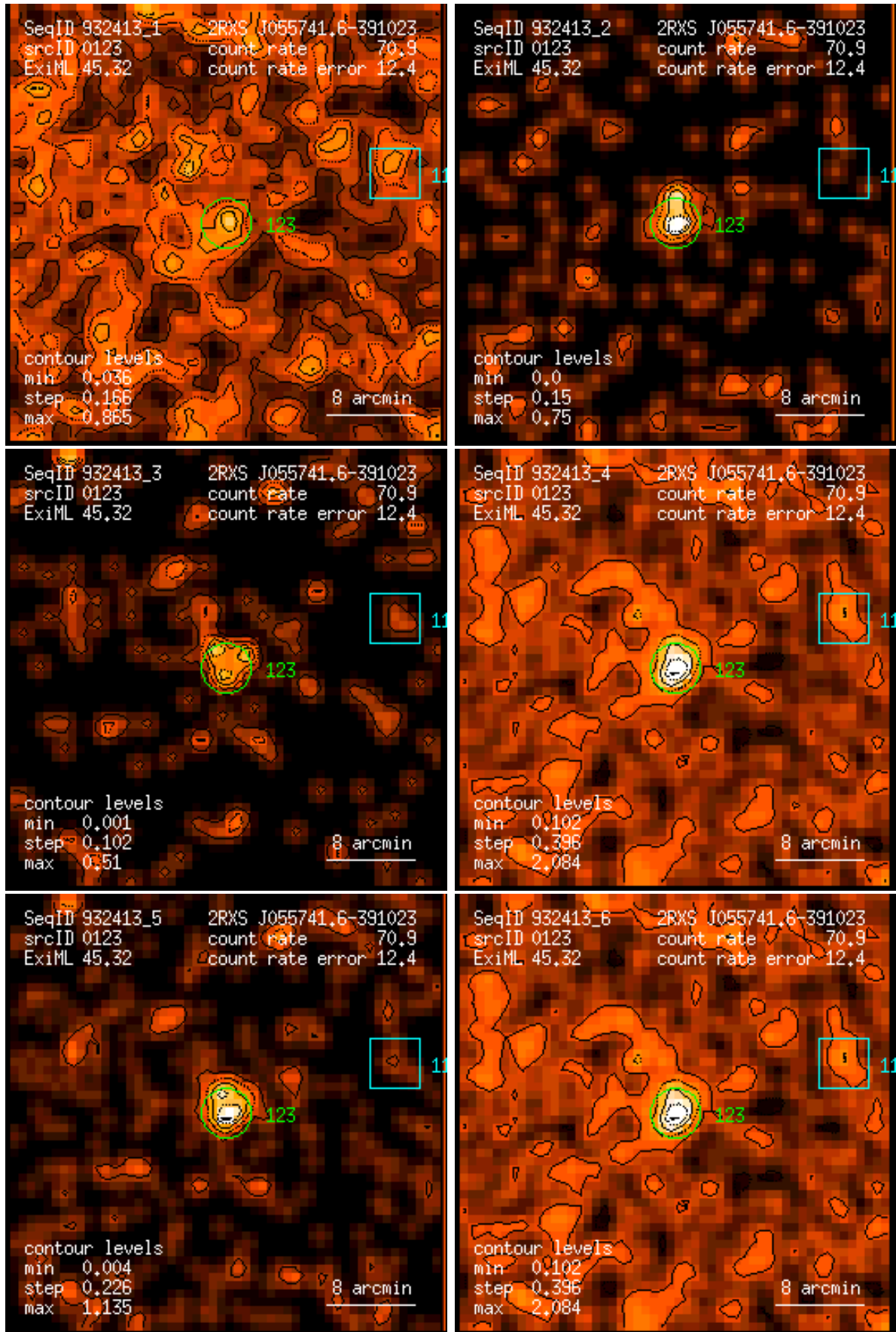
Figure 123: RASS 932413: detection 0123: band rate images, Gaussian filter: (1) PSPC channels 11 – 41, (2) 52 – 90, (3) 91 – 201, (4) 11 – 235, (5) 52 – 201, (6) 11 – 201. Broad band rates in counts/ks. Band rate contour levels in counts/ks/arcmin 2 .
