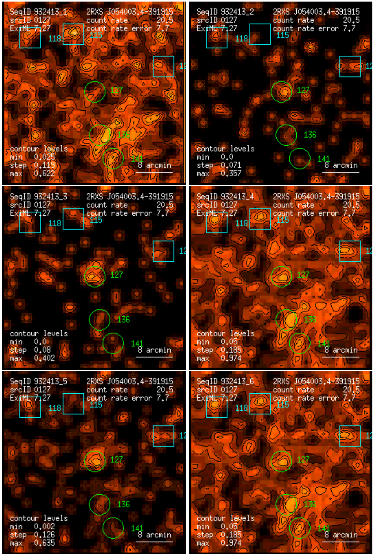
Figure 127: RASS 932413: detection 0127: band rate images, Gaussian filter: (1) PSPC channels 11 – 41, (2) 52 – 90, (3) 91 – 201, (4) 11 – 235, (5) 52 – 201, (6) 11 – 201. Broad band rates in counts/ks. Band rate contour levels in counts/ks/arcmin 2 .
