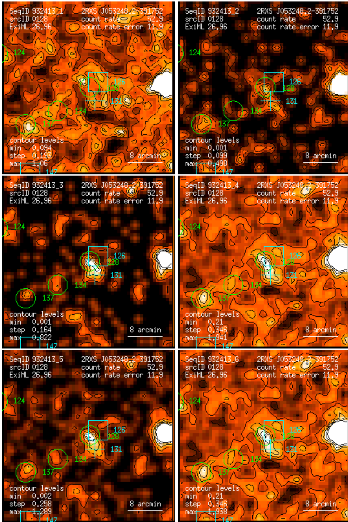
Figure 128: RASS 932413: detection 0128: band rate images, Gaussian filter: (1) PSPC channels 11 – 41, (2) 52 – 90, (3) 91 – 201, (4) 11 – 235, (5) 52 – 201, (6) 11 – 201. Broad band rates in counts/ks. Band rate contour levels in counts/ks/arcmin 2 .
