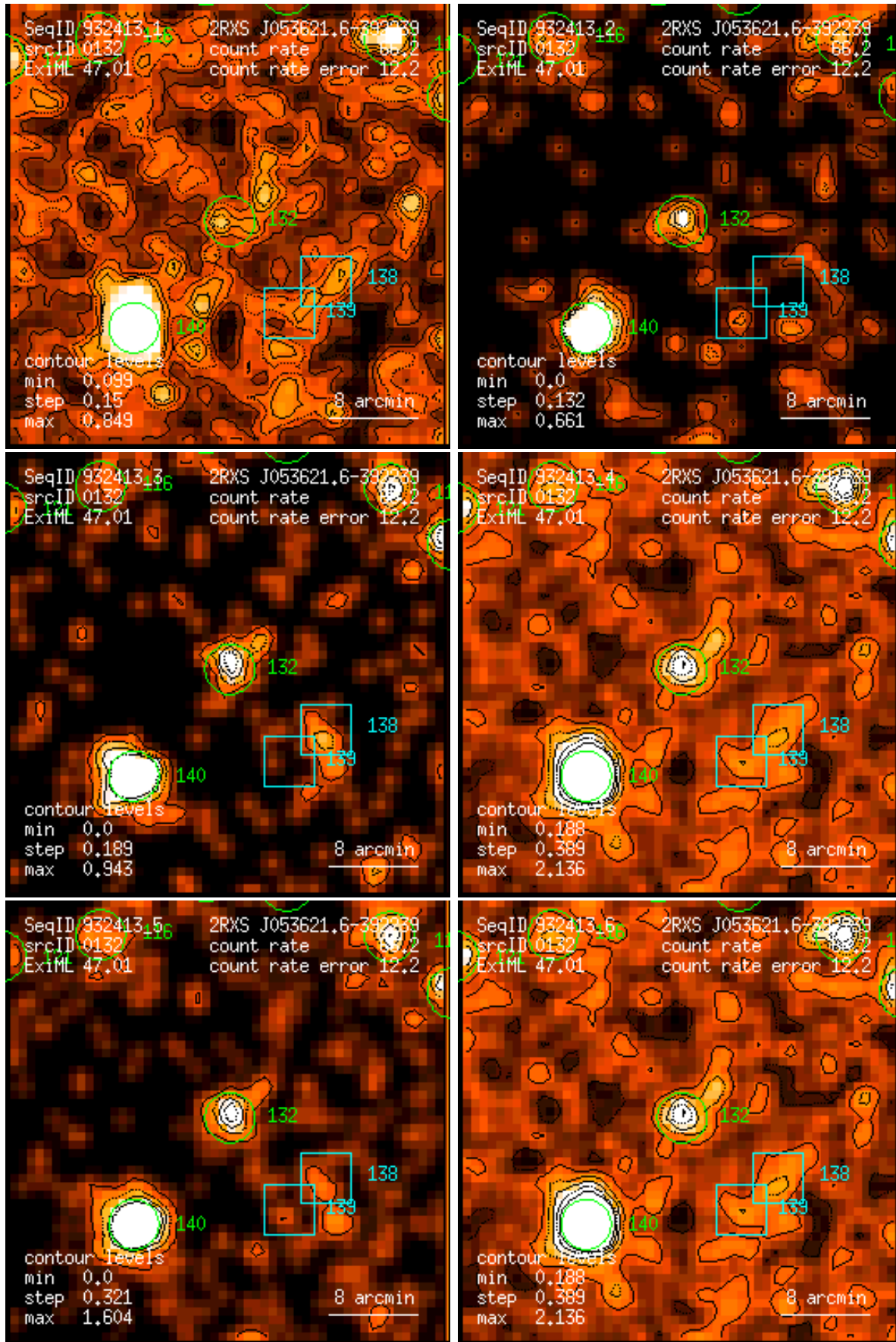
Figure 132: RASS 932413: detection 0132: band rate images, Gaussian filter: (1) PSPC channels 11 – 41, (2) 52 – 90, (3) 91 – 201, (4) 11 – 235, (5) 52 – 201, (6) 11 – 201. Broad band rates in counts/ks. Band rate contour levels in counts/ks/arcmin 2 .
