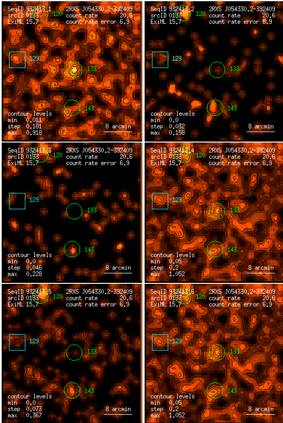
Figure 133: RASS 932413: detection 0133: band rate images, Gaussian filter: (1) PSPC channels 11 – 41, (2) 52 – 90, (3) 91 – 201, (4) 11 – 235, (5) 52 – 201, (6) 11 – 201. Broad band rates in counts/ks. Band rate contour levels in counts/ks/arcmin 2 .
