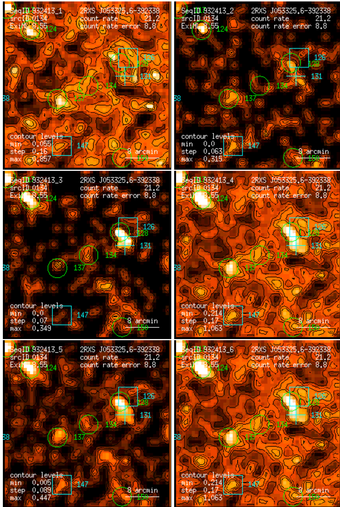
Figure 134: RASS 932413: detection 0134: band rate images, Gaussian filter: (1) PSPC channels 11 – 41, (2) 52 – 90, (3) 91 – 201, (4) 11 – 235, (5) 52 – 201, (6) 11 – 201. Broad band rates in counts/ks. Band rate contour levels in counts/ks/arcmin 2 .
