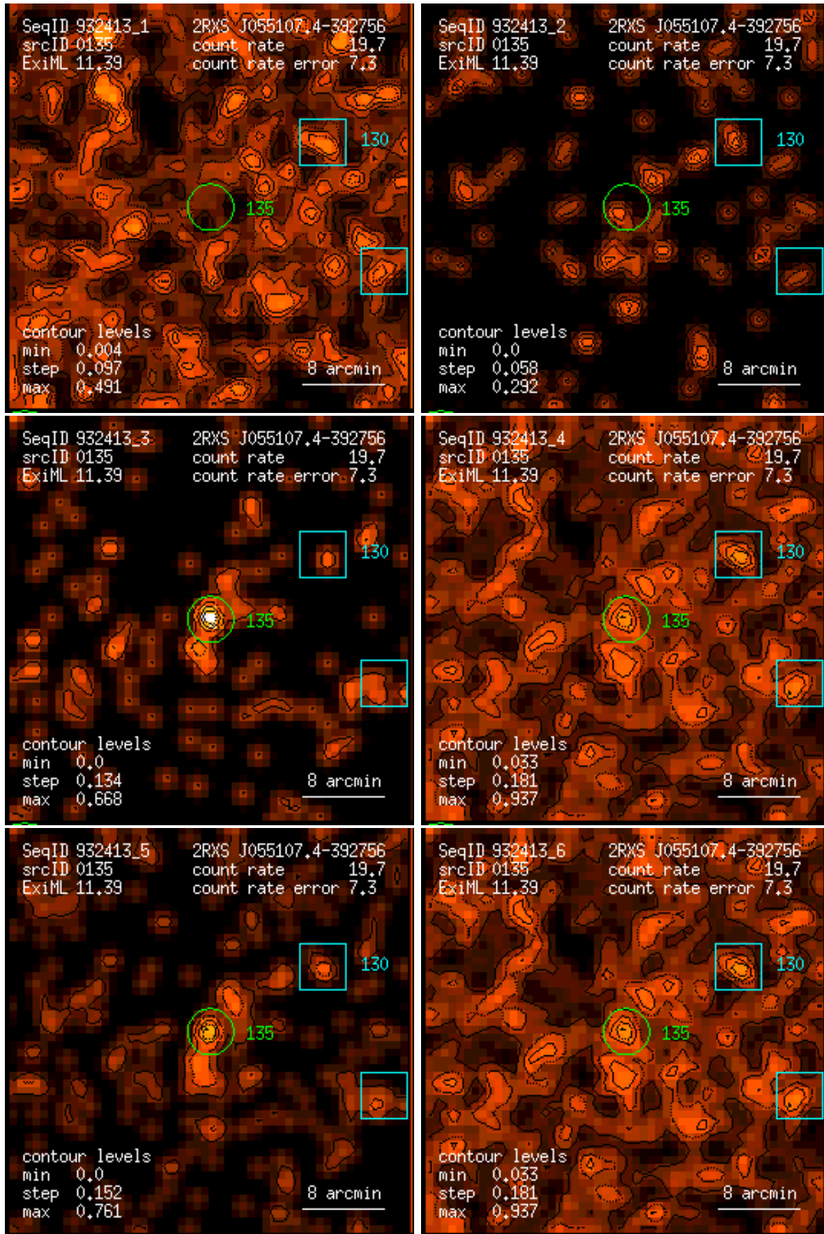
Figure 135: RASS 932413: detection 0135: band rate images, Gaussian filter: (1) PSPC channels 11 – 41, (2) 52 – 90, (3) 91 – 201, (4) 11 – 235, (5) 52 – 201, (6) 11 – 201. Broad band rates in counts/ks. Band rate contour levels in counts/ks/arcmin 2 .
