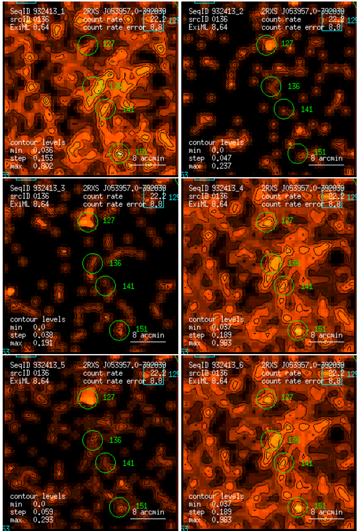
Figure 136: RASS 932413: detection 0136: band rate images, Gaussian filter: (1) PSPC channels 11 – 41, (2) 52 – 90, (3) 91 – 201, (4) 11 – 235, (5) 52 – 201, (6) 11 – 201. Broad band rates in counts/ks. Band rate contour levels in counts/ks/arcmin 2 .
