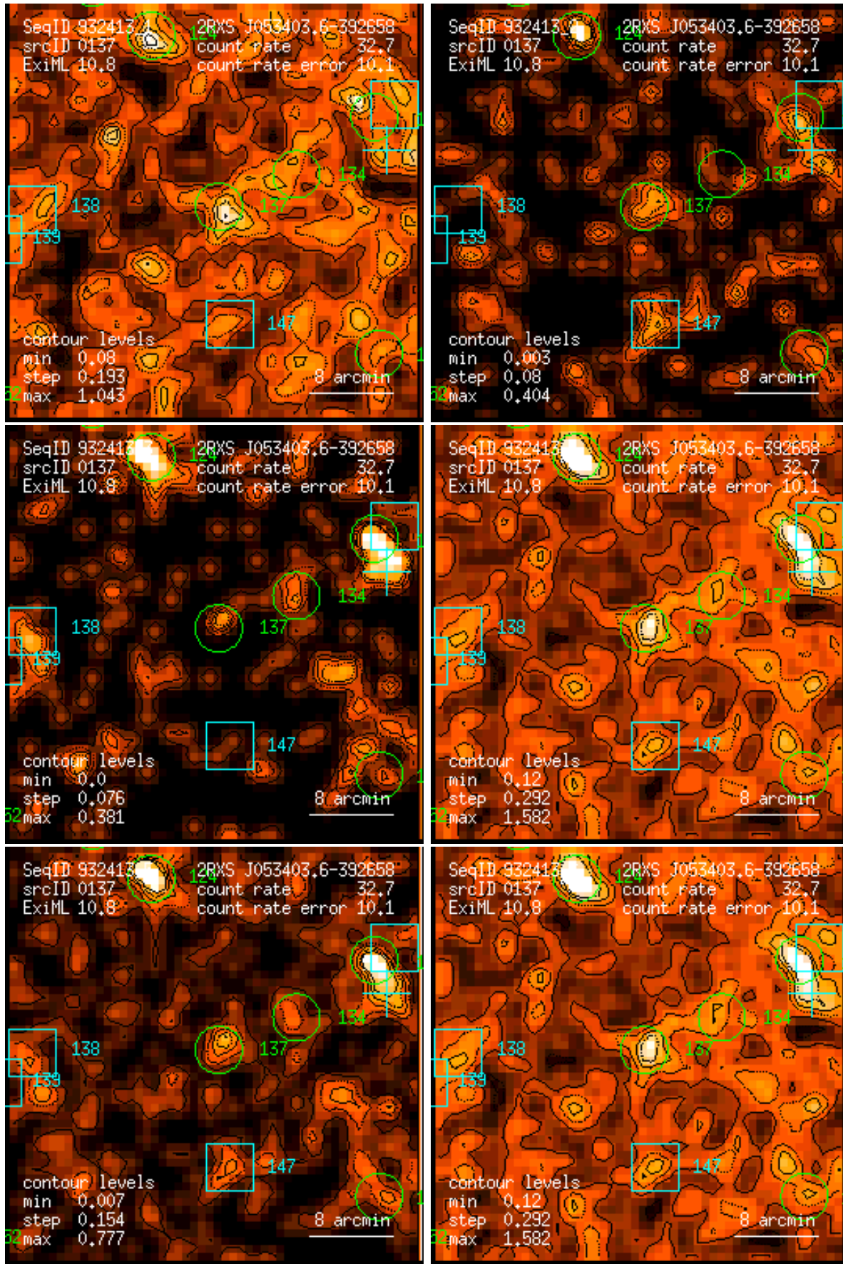
Figure 137: RASS 932413: detection 0137: band rate images, Gaussian filter: (1) PSPC channels 11 – 41, (2) 52 – 90, (3) 91 – 201, (4) 11 – 235, (5) 52 – 201, (6) 11 – 201. Broad band rates in counts/ks. Band rate contour levels in counts/ks/arcmin 2 .
