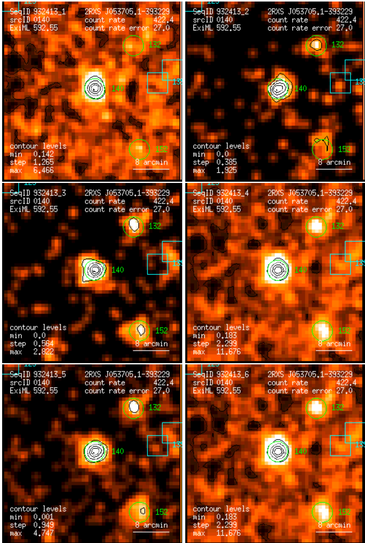
Figure 140: RASS 932413: detection 0140: band rate images, Gaussian filter: (1) PSPC channels 11 – 41, (2) 52 – 90, (3) 91 – 201, (4) 11 – 235, (5) 52 – 201, (6) 11 – 201. Broad band rates in counts/ks. Band rate contour levels in counts/ks/arcmin 2 .
