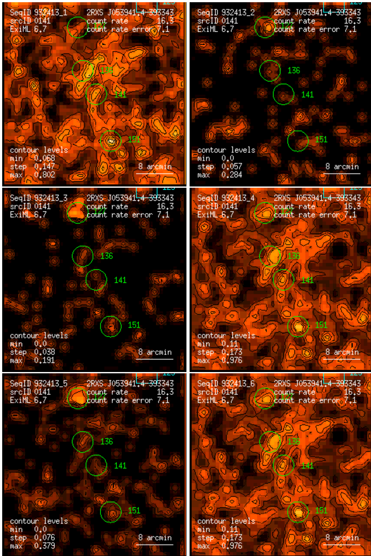
Figure 141: RASS 932413: detection 0141: band rate images, Gaussian filter: (1) PSPC channels 11 – 41, (2) 52 – 90, (3) 91 – 201, (4) 11 – 235, (5) 52 – 201, (6) 11 – 201. Broad band rates in counts/ks. Band rate contour levels in counts/ks/arcmin 2 .
