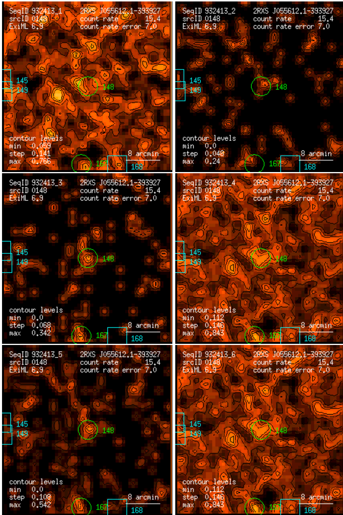
Figure 148: RASS 932413: detection 0148: band rate images, Gaussian filter: (1) PSPC channels 11 – 41, (2) 52 – 90, (3) 91 – 201, (4) 11 – 235, (5) 52 – 201, (6) 11 – 201. Broad band rates in counts/ks. Band rate contour levels in counts/ks/arcmin 2 .
