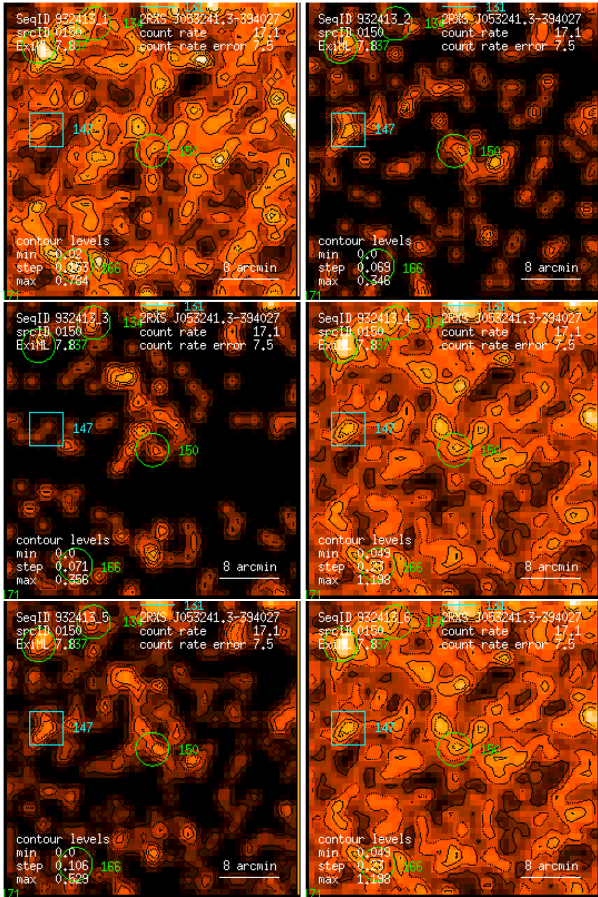
Figure 150: RASS 932413: detection 0150: band rate images, Gaussian filter: (1) PSPC channels 11 – 41, (2) 52 – 90, (3) 91 – 201, (4) 11 – 235, (5) 52 – 201, (6) 11 – 201. Broad band rates in counts/ks. Band rate contour levels in counts/ks/arcmin 2 .
