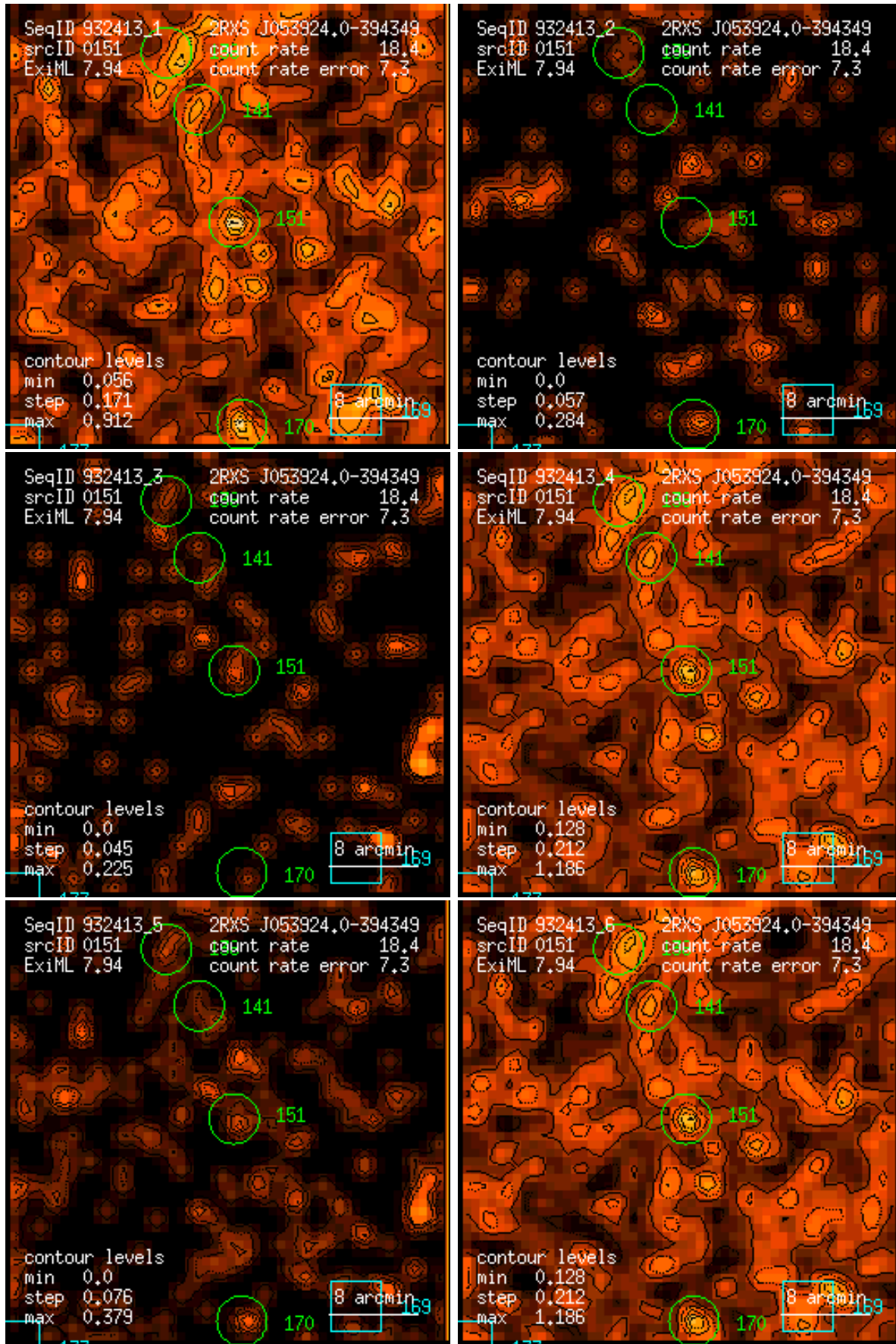
Figure 151: RASS 932413: detection 0151: band rate images, Gaussian filter: (1) PSPC channels 11 – 41, (2) 52 – 90, (3) 91 – 201, (4) 11 – 235, (5) 52 – 201, (6) 11 – 201. Broad band rates in counts/ks. Band rate contour levels in counts/ks/arcmin 2 .
