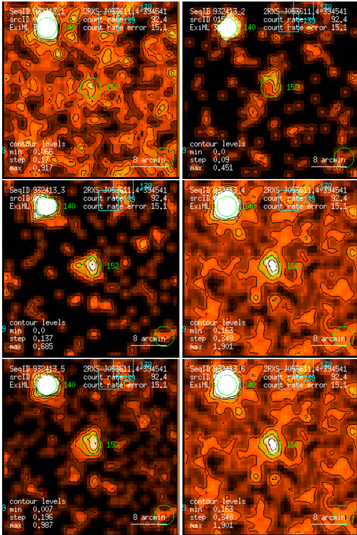
Figure 152: RASS 932413: detection 0152: band rate images, Gaussian filter: (1) PSPC channels 11 – 41, (2) 52 – 90, (3) 91 – 201, (4) 11 – 235, (5) 52 – 201, (6) 11 – 201. Broad band rates in counts/ks. Band rate contour levels in counts/ks/arcmin 2 .
