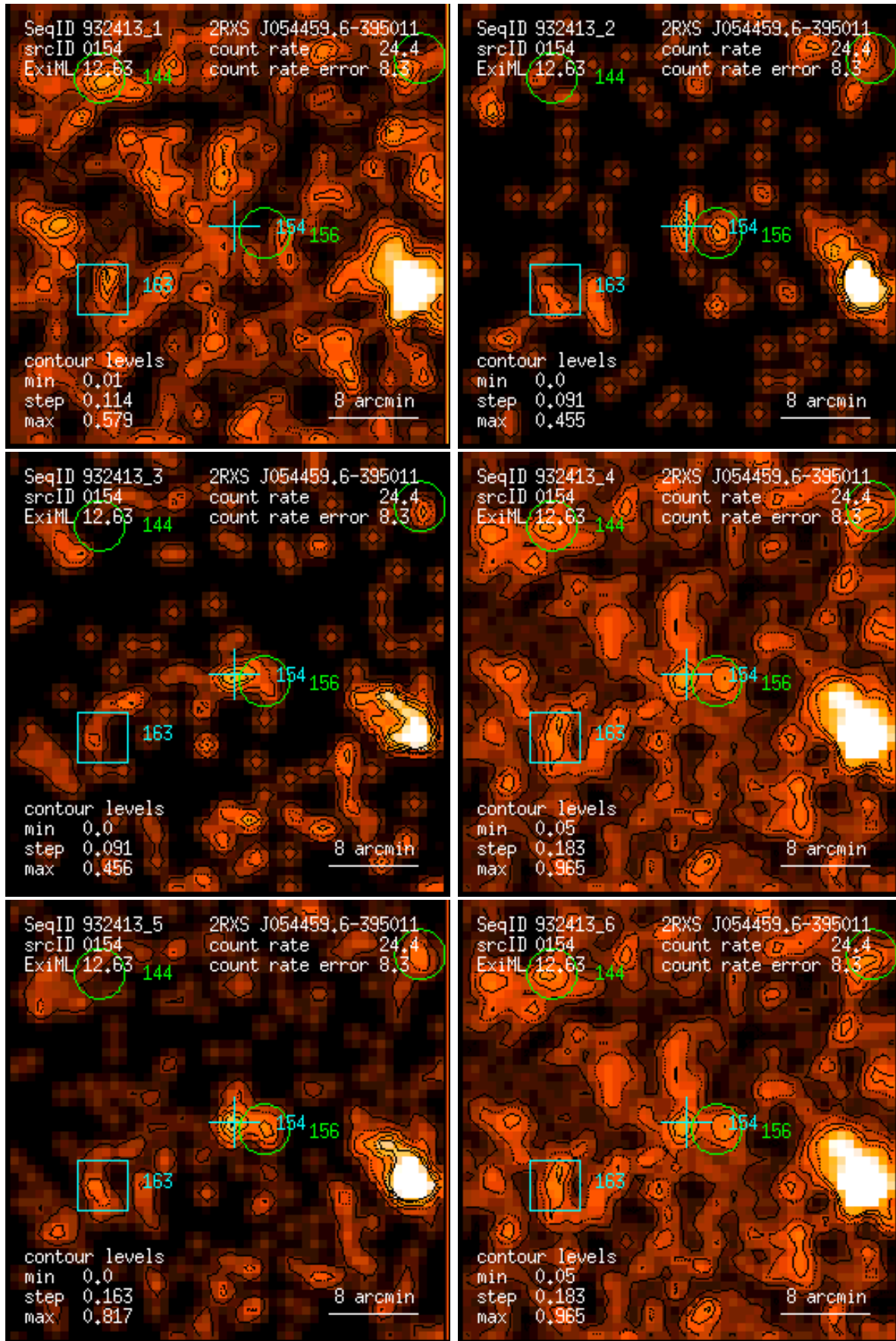
Figure 154: RASS 932413: detection 0154: band rate images, Gaussian filter: (1) PSPC channels 11 – 41, (2) 52 – 90, (3) 91 – 201, (4) 11 – 235, (5) 52 – 201, (6) 11 – 201. Broad band rates in counts/ks. Band rate contour levels in counts/ks/arcmin 2 .
