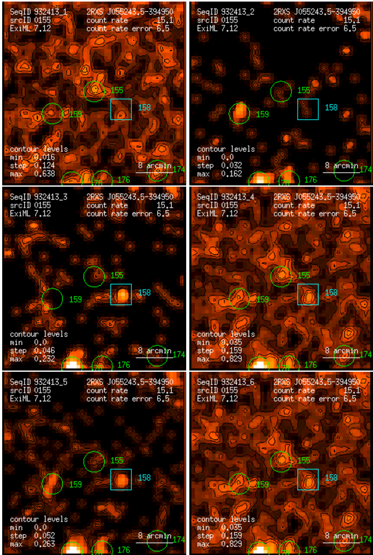
Figure 155: RASS 932413: detection 0155: band rate images, Gaussian filter: (1) PSPC channels 11 – 41, (2) 52 – 90, (3) 91 – 201, (4) 11 – 235, (5) 52 – 201, (6) 11 – 201. Broad band rates in counts/ks. Band rate contour levels in counts/ks/arcmin 2 .
