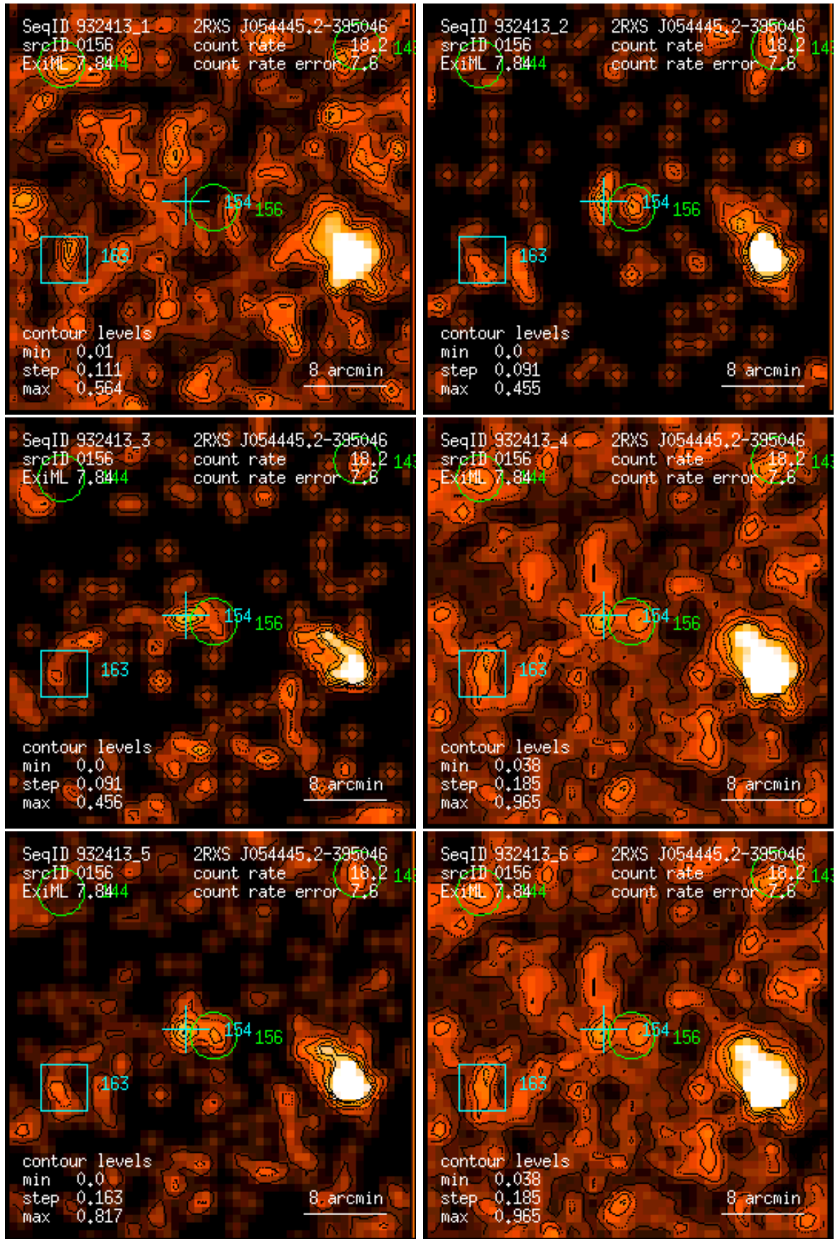
Figure 156: RASS 932413: detection 0156: band rate images, Gaussian filter: (1) PSPC channels 11 – 41, (2) 52 – 90, (3) 91 – 201, (4) 11 – 235, (5) 52 – 201, (6) 11 – 201. Broad band rates in counts/ks. Band rate contour levels in counts/ks/arcmin 2 .
