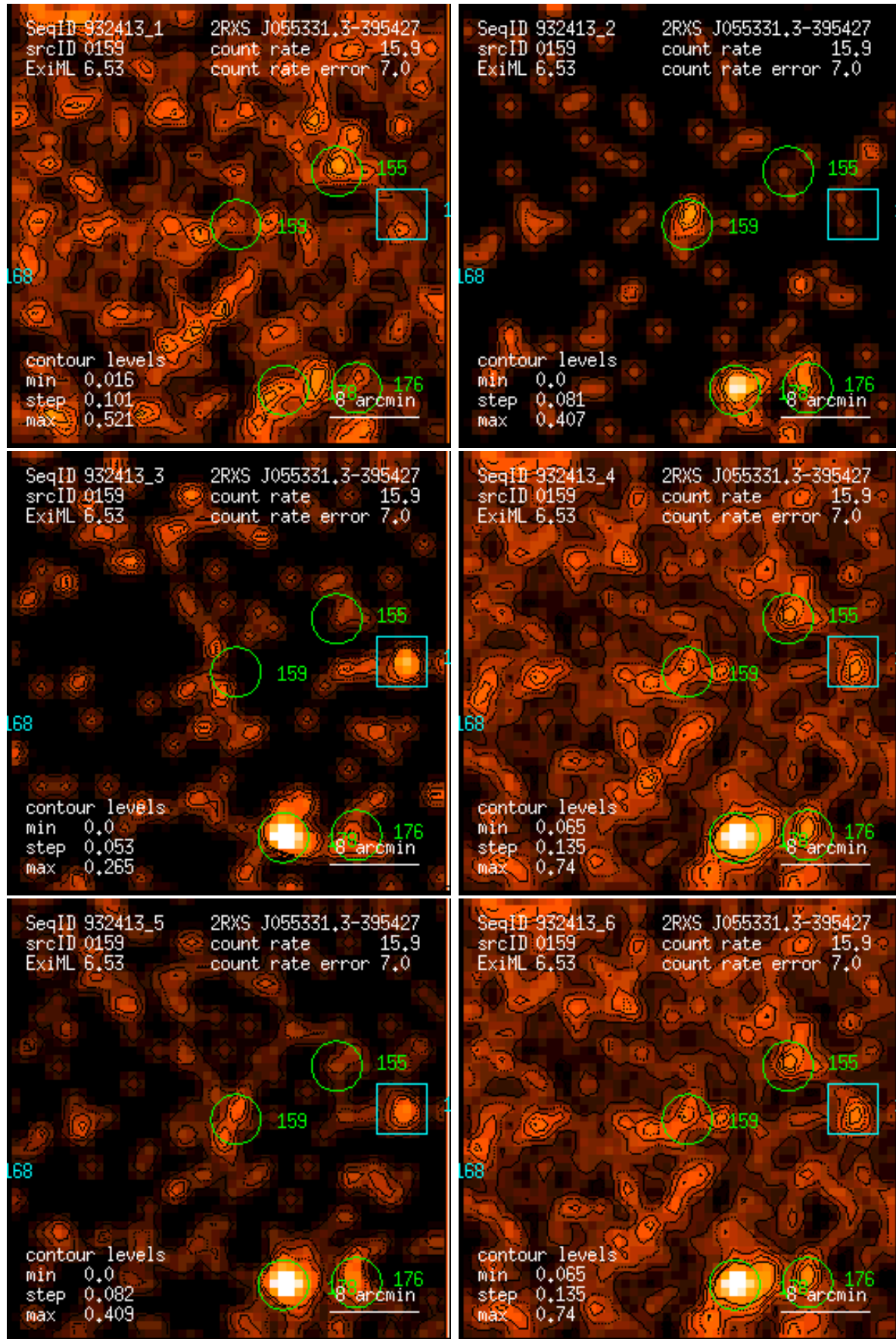
Figure 159: RASS 932413: detection 0159: band rate images, Gaussian filter: (1) PSPC channels 11 – 41, (2) 52 – 90, (3) 91 – 201, (4) 11 – 235, (5) 52 – 201, (6) 11 – 201. Broad band rates in counts/ks. Band rate contour levels in counts/ks/arcmin 2 .
