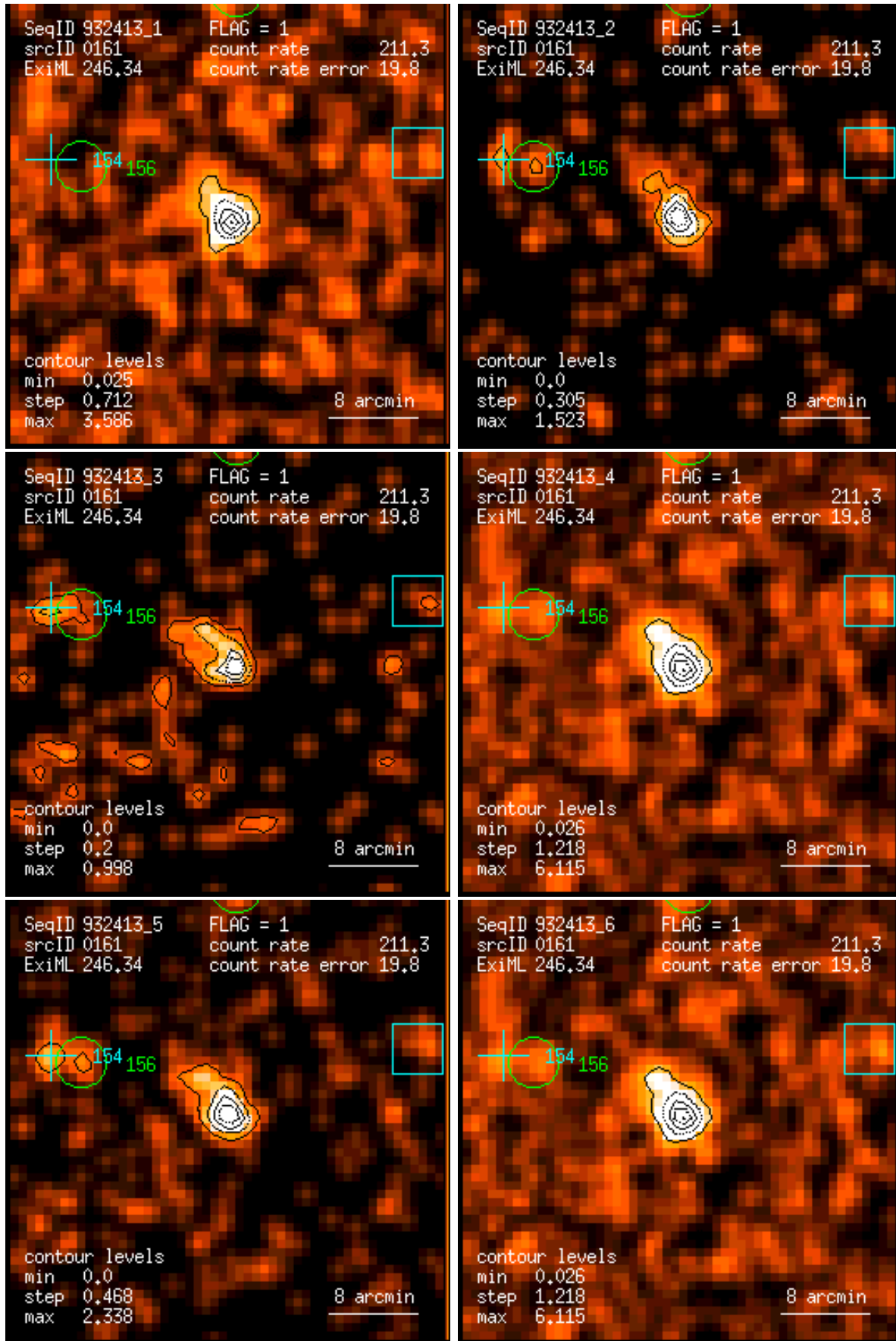
Figure 161: RASS 932413: detection 0161: band rate images, Gaussian filter: (1) PSPC channels 11 – 41, (2) 52 – 90, (3) 91 – 201, (4) 11 – 235, (5) 52 – 201, (6) 11 – 201. Broad band rates in counts/ks. Band rate contour levels in counts/ks/arcmin 2 .
