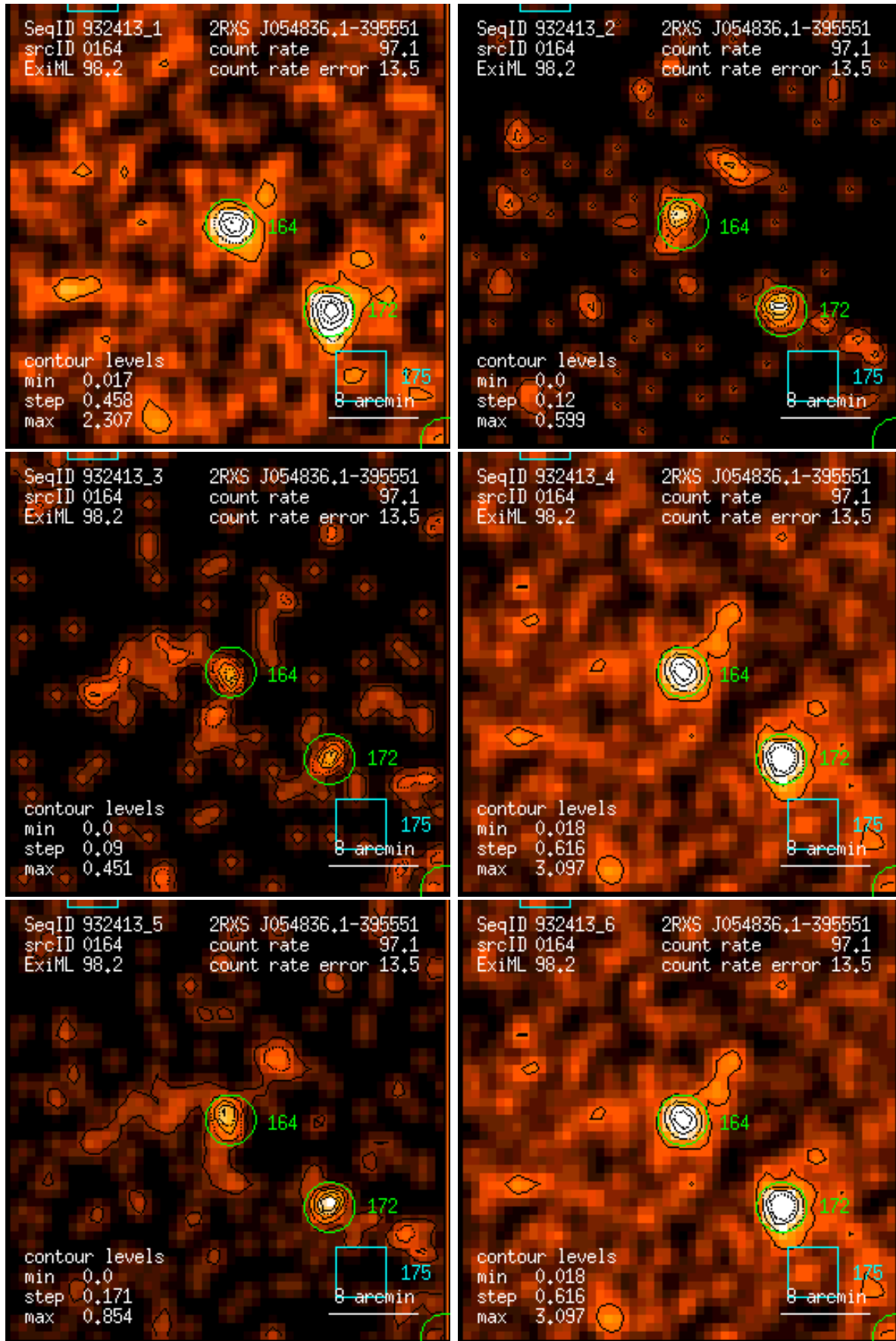
Figure 164: RASS 932413: detection 0164: band rate images, Gaussian filter: (1) PSPC channels 11 – 41, (2) 52 – 90, (3) 91 – 201, (4) 11 – 235, (5) 52 – 201, (6) 11 – 201. Broad band rates in counts/ks. Band rate contour levels in counts/ks/arcmin 2 .
