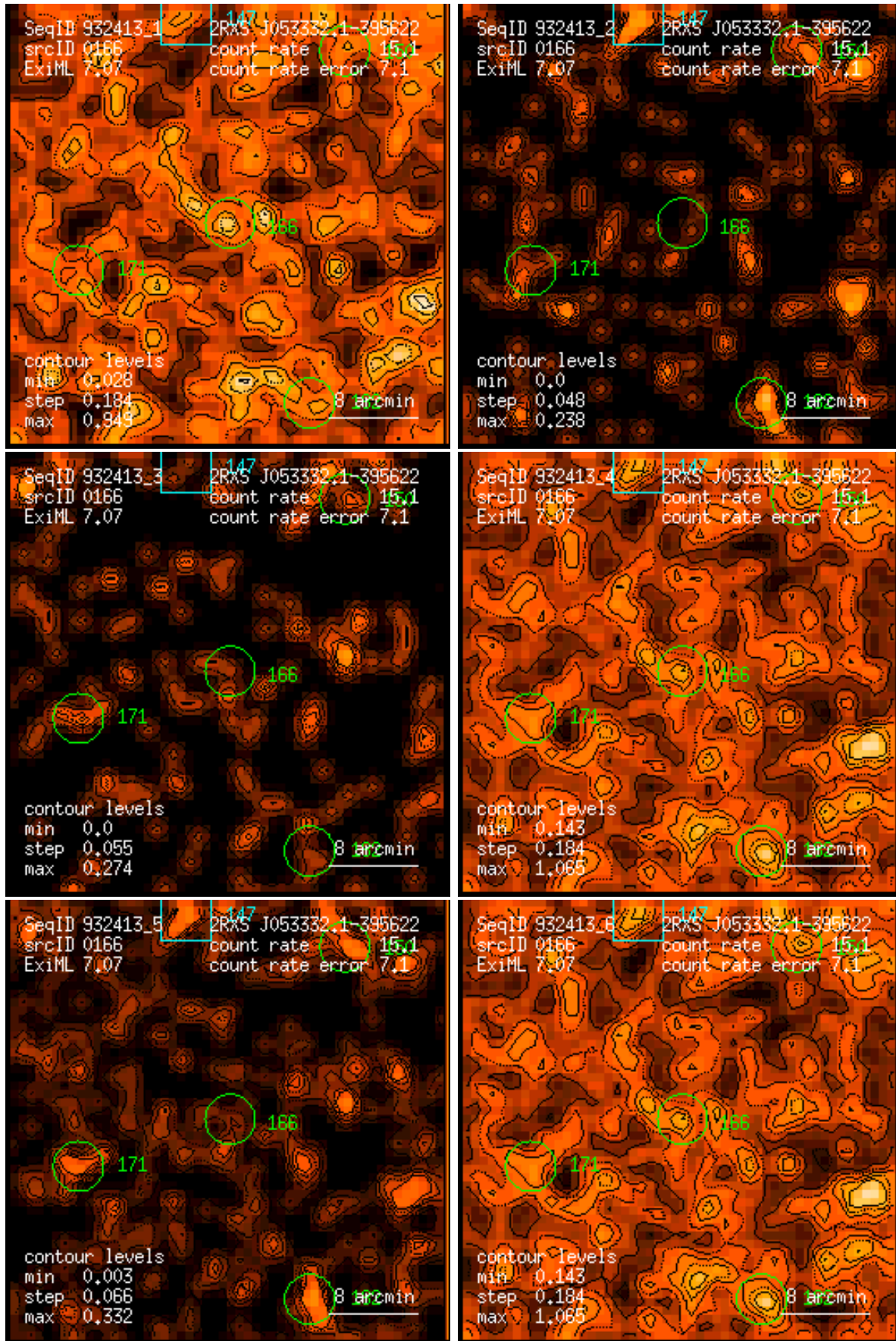
Figure 166: RASS 932413: detection 0166: band rate images, Gaussian filter: (1) PSPC channels 11 – 41, (2) 52 – 90, (3) 91 – 201, (4) 11 – 235, (5) 52 – 201, (6) 11 – 201. Broad band rates in counts/ks. Band rate contour levels in counts/ks/arcmin 2 .
