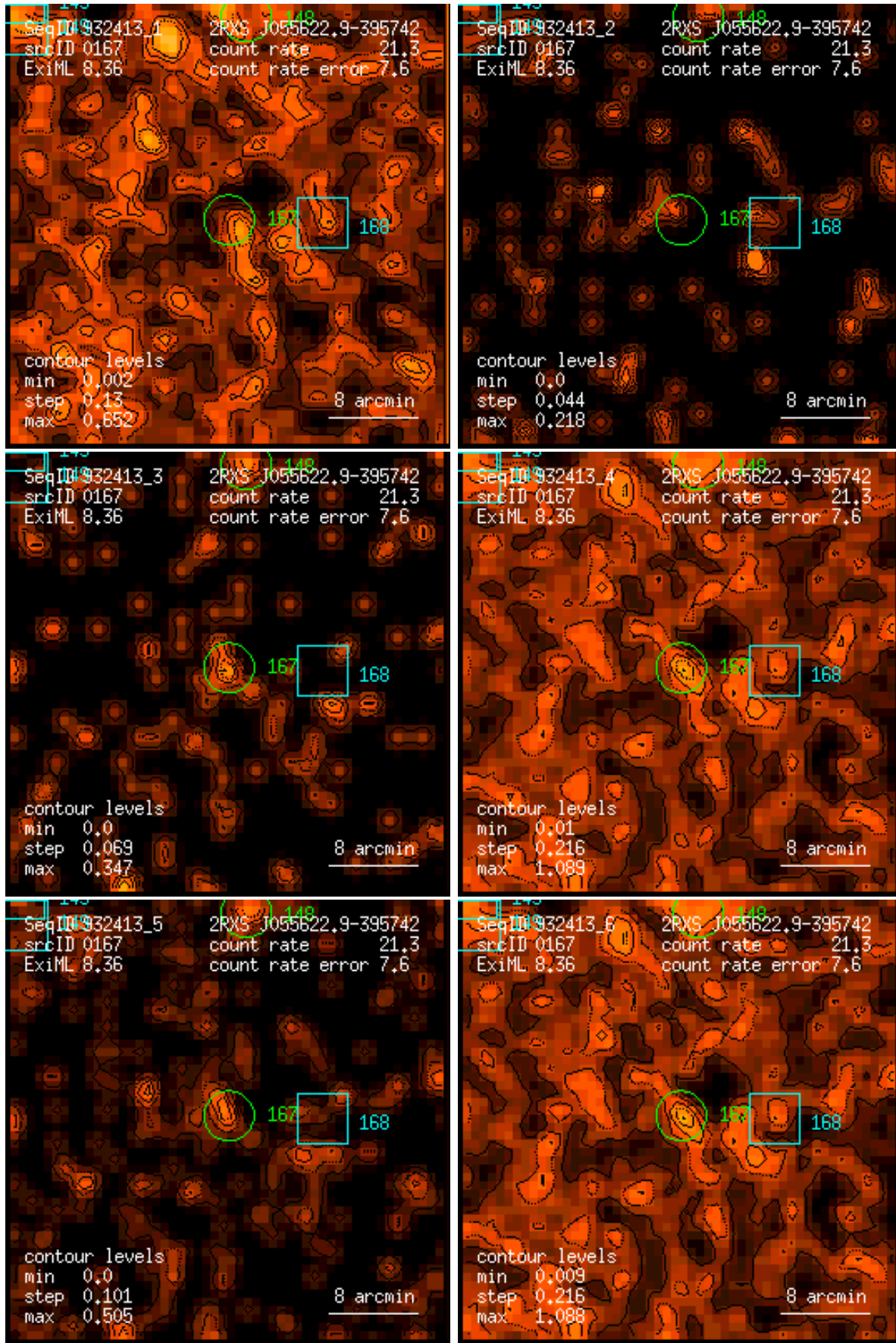
Figure 167: RASS 932413: detection 0167: band rate images, Gaussian filter: (1) PSPC channels 11 – 41, (2) 52 – 90, (3) 91 – 201, (4) 11 – 235, (5) 52 – 201, (6) 11 – 201. Broad band rates in counts/ks. Band rate contour levels in counts/ks/arcmin 2 .
